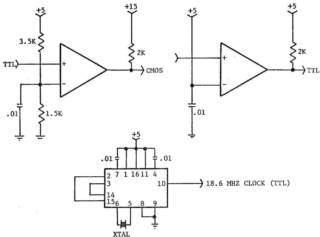
Figure 7.2-1 Translator Circuitry.
