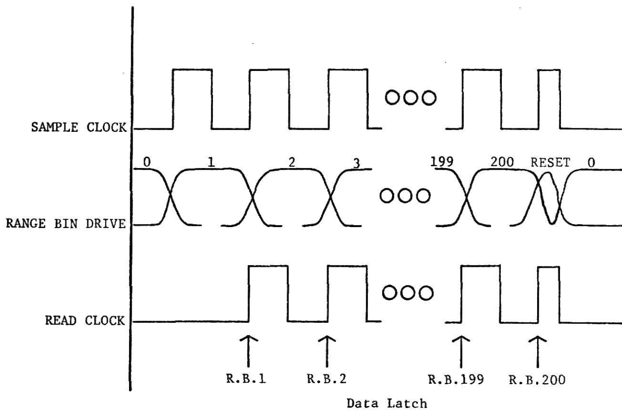
Figure 4.4-1 Timing of READ and SAMPLE CLOCK
