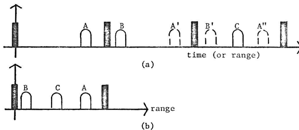
Figure 2.2-2 Multiple-time-around Echoes.
