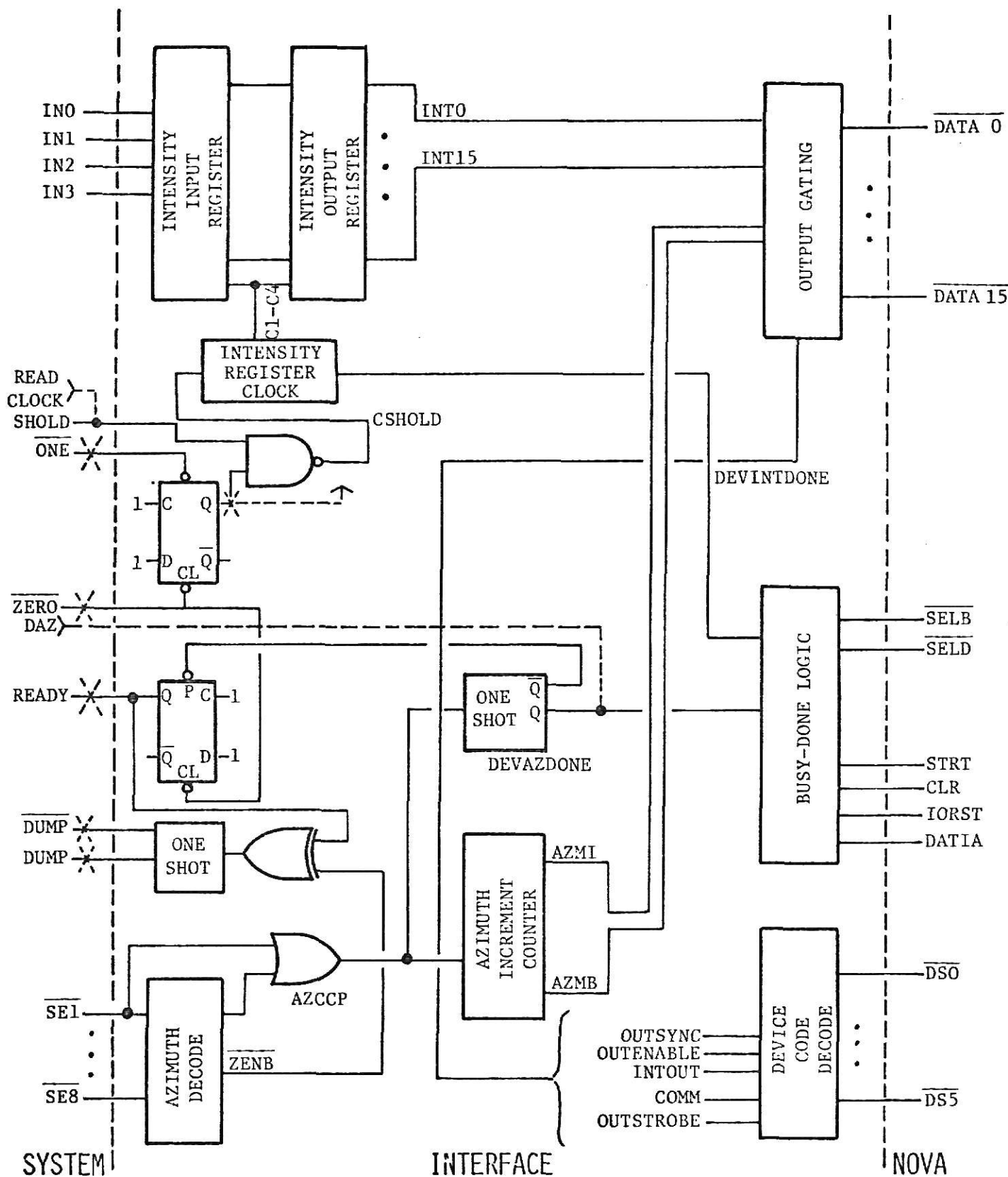
Figure 9.1 Modifications to Existing Processor.
