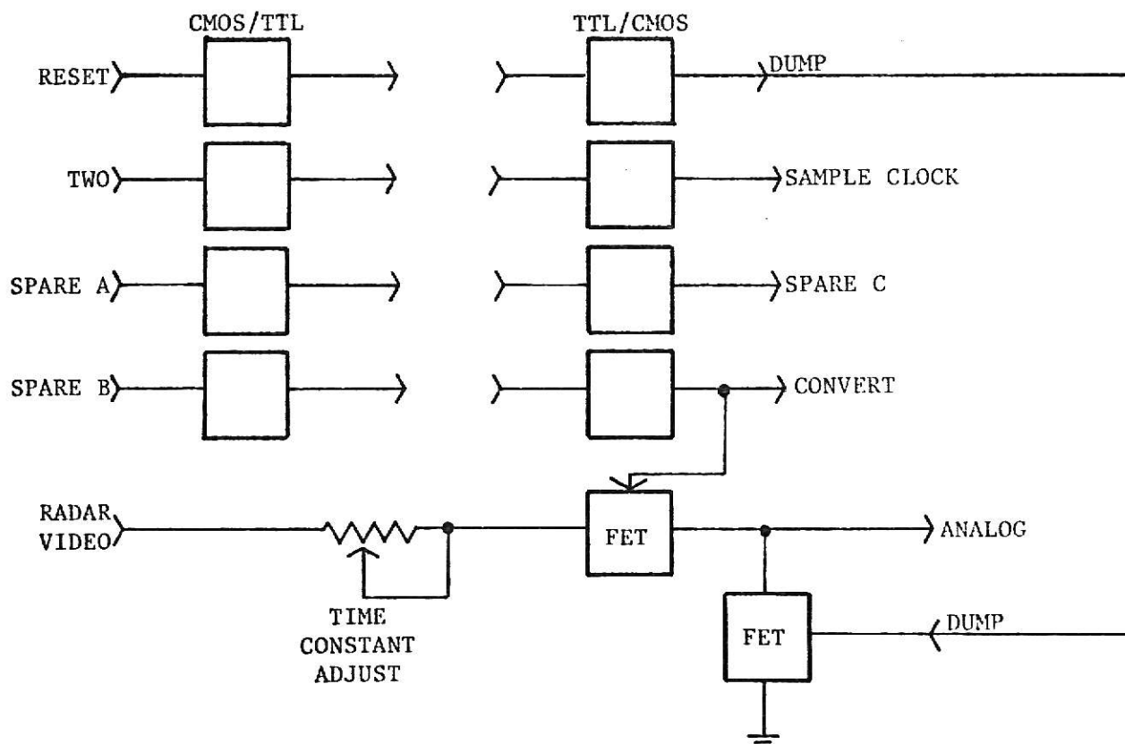
Figure 7.2-2 Translator Block Diagram.
