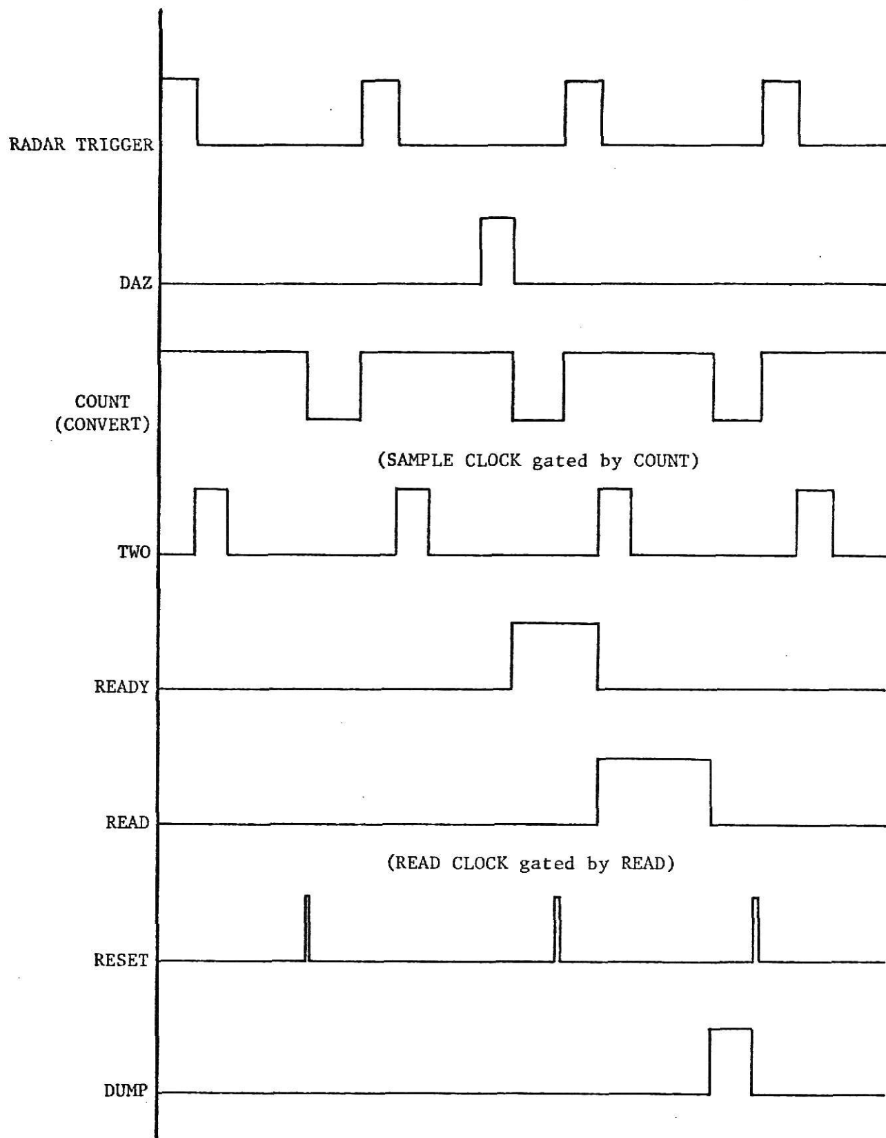
Figure 3.3-1 I &amp; Q Timing Diagram.
