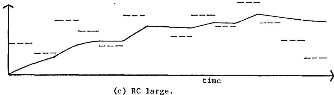
Figure 5.3-1 R-C Integration.
