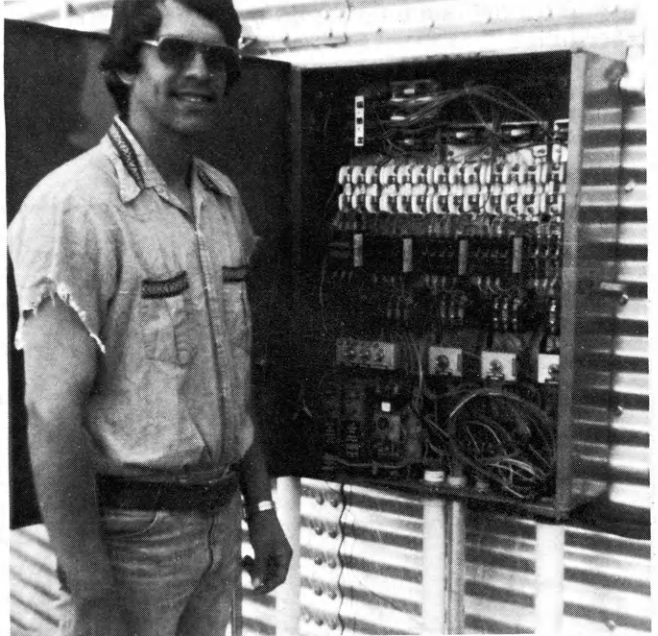
The control panel is the nerve center for the drying system; it controls the burners and fills and unloads the automatic grain dryer.
