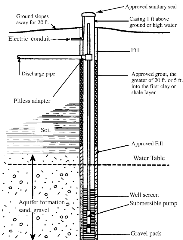
Figure 3. Required well construction — unconfined aquifer
