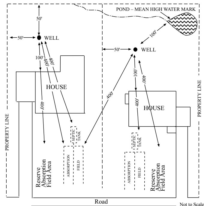
Figure 2. Ideal private well location
