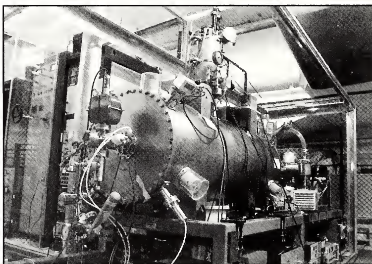
The K-State CRYEBIS particle accelerator is one of the few in the United States. It has a maximum acceleration voltage of 7.5 million volts. (Photo by David Mayes)
