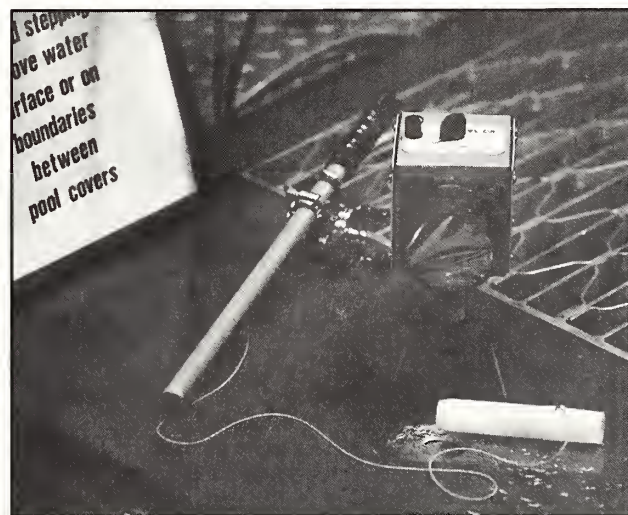
Students use both a "fishing rod" to lower samples into the core of the accelerator and a hand-held radiation device when working with the TRIGA Mark II. (Photo by Brad Camp)
