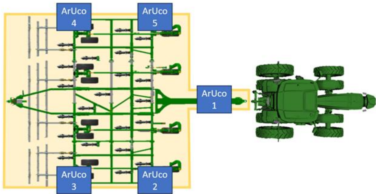
Figure 2.2 Placement of the ArUco markers on the physical implement
