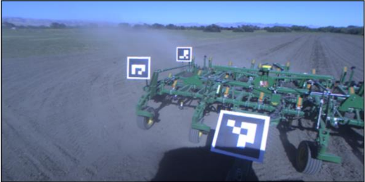
Figure 2.6 Not all markers present in camera field of view during turn
