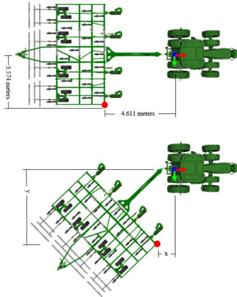
Figure 2.10 Point position estimation error induced by implement pivot point
