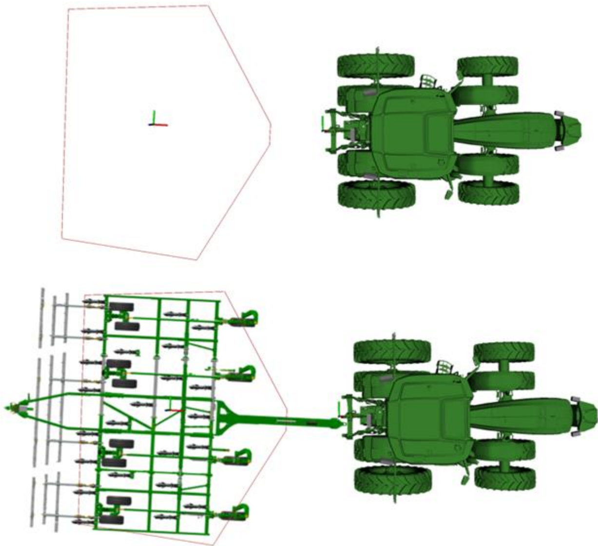
Figure 2.12 RVIZ2 Visualization of newly defined implement boundary
