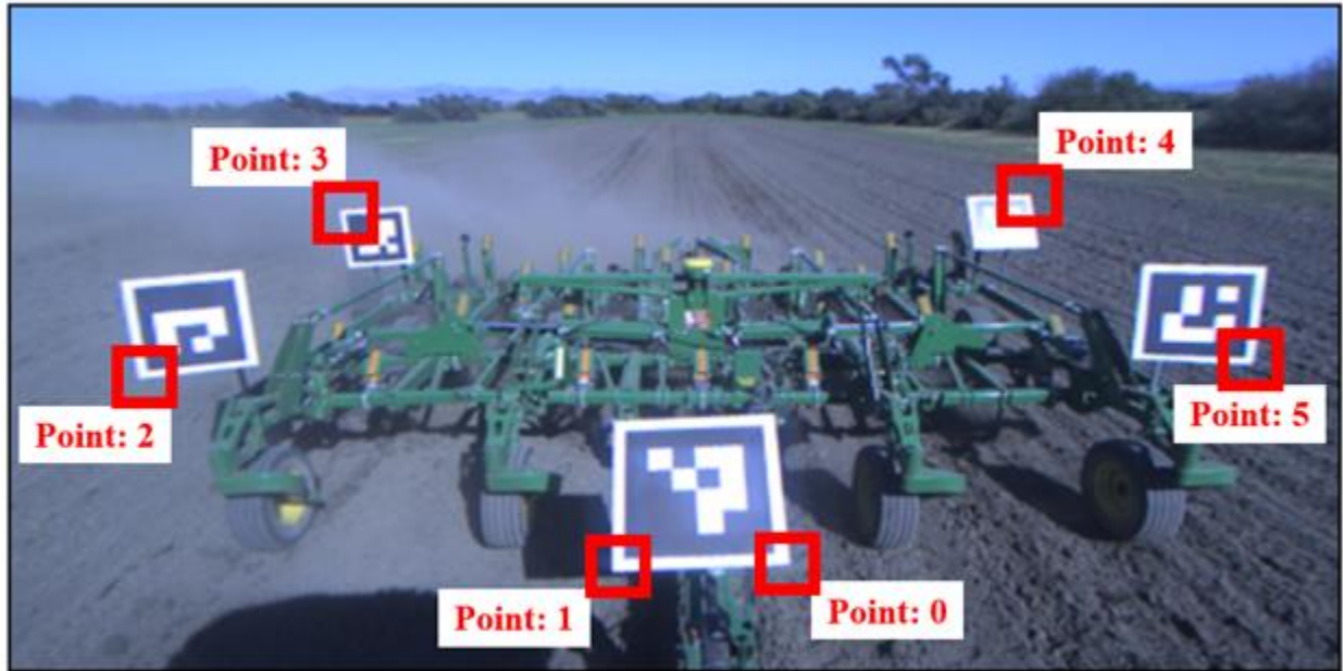
Figure 2.8 Specific pixels to be identified with detection algorithm
