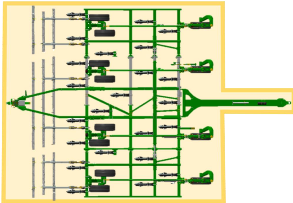
Figure 2.1 Visualizing the implement boundary in dark yellow and implement footprint in light yellow
