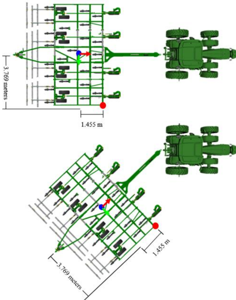
Figure 2.11 Transformed point location in three-dimensions with respect to implement origin
