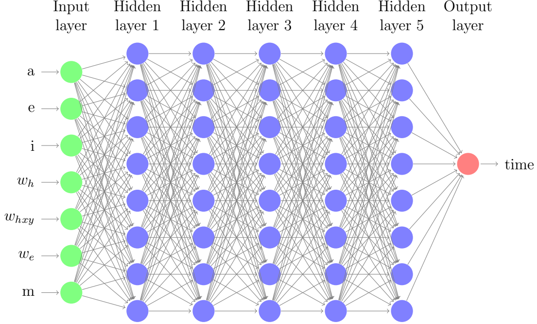
Figure 5.2: Example of DNN-5 with 40 neurons (an 8-8-8-8-8 configuration).
