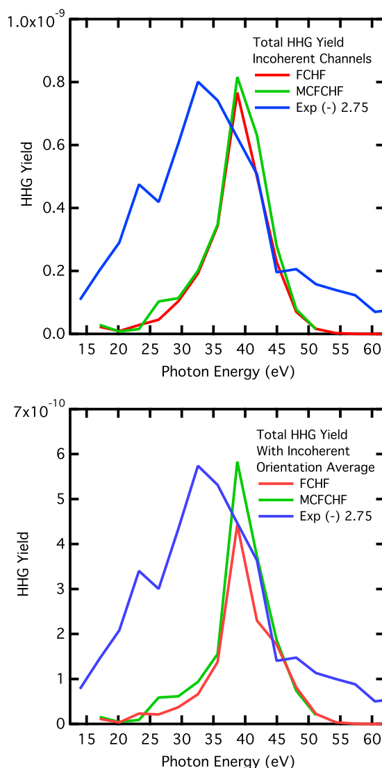
FIG. 8. Top panel: The total of the QRS results from the three outermost valence orbitals of \text{SF}_6 shown in the middle column in Fig. 6. Bottom panel: The corresponding total of the incoherent orientation averages shown in the right panel in Fig. 6. The results in both panels are compared to the experimental HHG spectrum at 4.0 \times 10^{14} \text{ W/cm}^2 with the focal point at (-) 2.75 mm. The experimental scale is arbitrary and selected so that the maximum HHG yield is the same as the MCFCHF QRS results.
