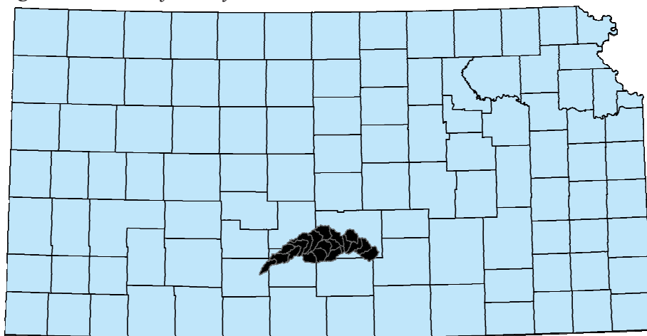
Figure 1. Location of Cheney Lake watershed in Kansas.
