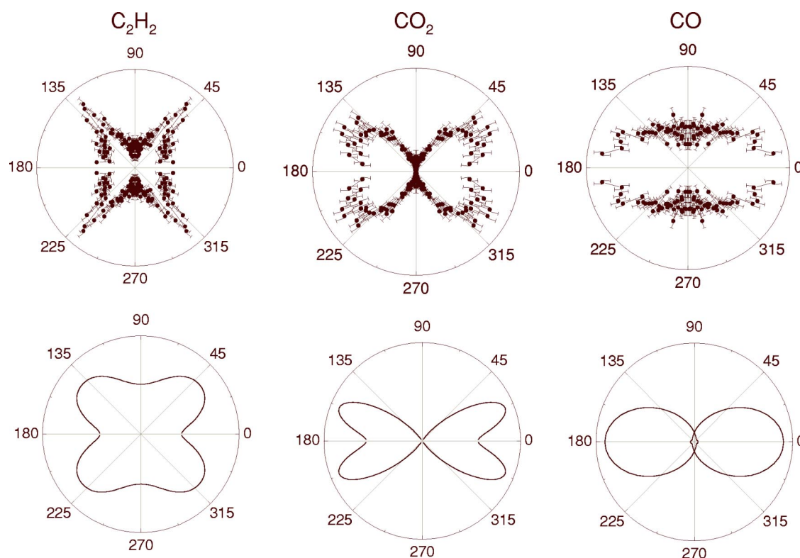
FIG. 1. (Color online). Experimental angular distributions for pairs of singly charged fragments detected in coincidence. Distributions were measured for \text{C}_2\text{H}_2^{2+} \rightarrow \text{CH}^+ + \text{CH}^+ , \text{CO}^{2+} \rightarrow \text{C}^+ + \text{O}^+ ; \text{CO}_2^{2+} \rightarrow \text{CO}^+ + \text{O}^+ ; channels. Estimated pulse peak intensity is 6 \times 10^{13} \text{ W/cm}^2 , pulse duration is 8 fs, central wavelength is 800 nm, polarization is horizontal. Presented below are the angular-dependent single-ionization rates for neutral molecules calculated using Molecular ADK theory for electric field of the same strength. For CO, the MO-ADK rate depends on orientation of the molecule and the symmetrized distribution is shown.
