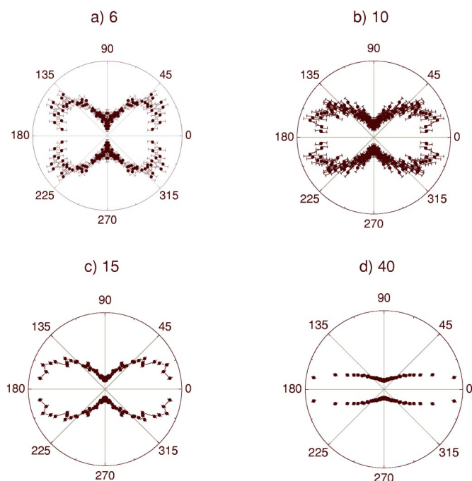
FIG. 2. (Color online). Experimental angular distributions for correlated ( \text{CO}^+ , \text{O}^+ ) ion pairs produced by dissociation of \text{CO}_2 by 8-fs (800-nm central wavelength) laser pulses. Laser polarization is horizontal. Estimated peak intensities are ( 10^{13} W/cm ^2 ): (a) 6; (b) 10; (c) 15; (d) 40.
