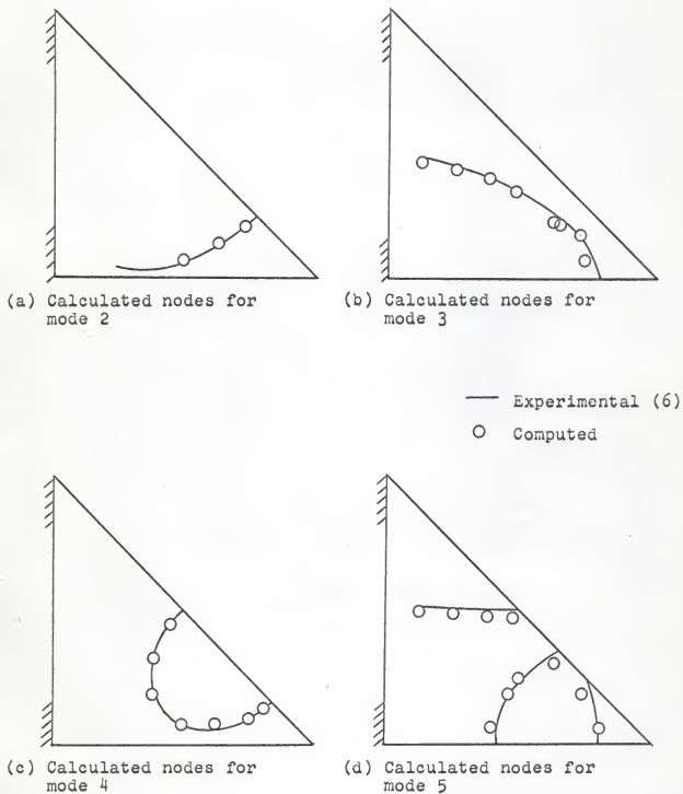
FIGURE 5. NODAL PATTERNS FOR PLATE B-0
