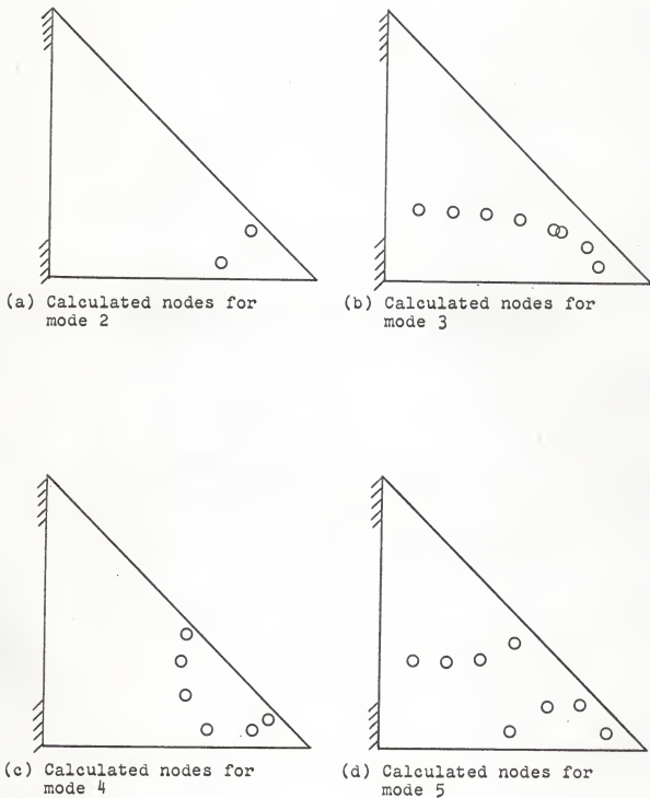
FIGURE 17. NODAL PATTERNS FOR PLATE B-8
