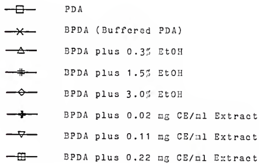
Fig. 36. Diameter of mycelial growth vs. days of culture for E. equiseti against CS3541 free extract and controls.
