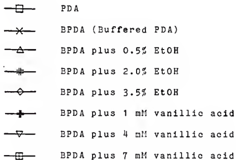
Fig. 59. Diameter of mycelial growth vs. days of culture for E. semitectum against vanillic acid and controls.
