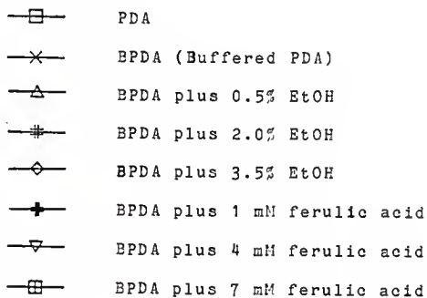
Fig. 56. Diameter of mycelial growth vs. days of culture for A. tenuissima cpx. against ferulic acid and controls.
