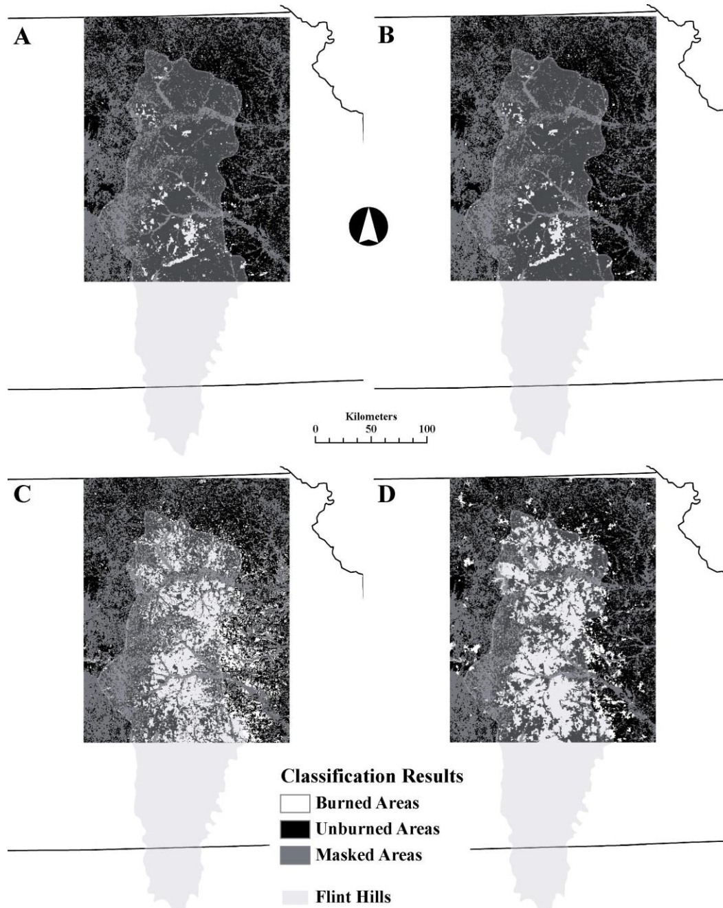
Figure 2: Classification results for Scenario #6 (red and NIR) from two imagery dates within the study period. Note the similarity between the pixel-based (A) and object-based (B) classification results from the April 2, 2008 image, compared to the difference between pixel (C) and object (D) classifications in the May 4, 2008 image.
