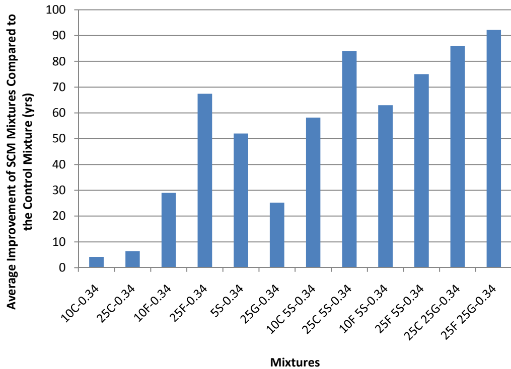
Figure 4.9 - Service life modeling predicted corrosion times
