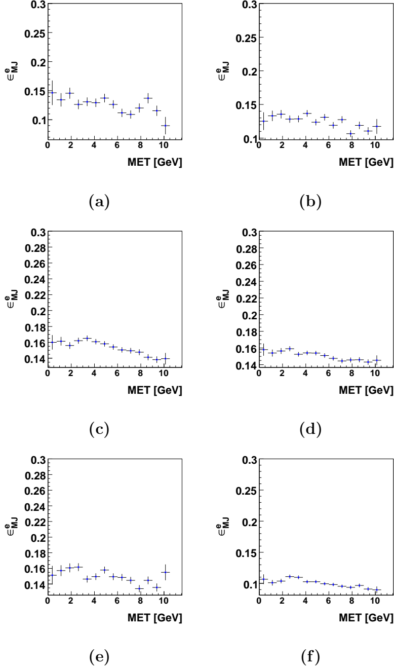
Figure 6.7: The electron mis-identification rate estimated from Jet-EM data sample as a function of \cancel{E}_T , (a) run range [ < 173101 ], (b) run range [ 173516-178721 ], (c) run range [ 178722-194568 ], (d) run range [ 194569-208122 ], (e) run range [ 208204-210711 ], (f) run range [ > 210835 ].
