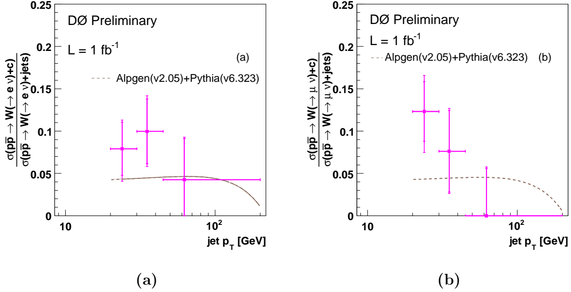
Figure 8.1: Measured ratio \frac{\sigma(p\bar{p} \rightarrow W+c\text{-jet})}{\sigma(p\bar{p} \rightarrow W+\text{jets})} as a function of jet p_T which is corrected to the particle level. (a) W \rightarrow e\nu mode, (b) W \rightarrow \mu\nu mode. Minimum threshold for the jet p_T is required to be 20 GeV and the pseudorapidity |\eta| < 2.0 in each p_T bin. The data points are shown with the theoretical expectation of ALPGEN+PYTHIA, where ALPGEN is for tree level matrix element calculation and PYTHIA is for the parton shower. Inner error bars represent the statistical only uncertainty on the measurement and the outer error bars corresponds to the total uncertainty where statistical and systematic uncertainties are added in quadrature.
