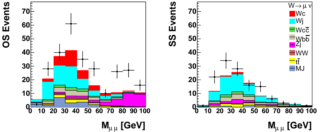
Figure 7.1: The distribution of invariant mass, M_{\mu\mu} , of two final state muons in the W(\rightarrow \mu\nu)+\mu -tagged jet sample before the cut M_{\mu\mu} < 70 GeV cut. The restriction on high invariant mass of two muons suppresses the Z background. Events with the isolated muon charge opposite (equal) to that the muon present in the jet, OS events (SS events), are shown on the left (right) side. The total MC prediction is the sum of the expectations from the W + c -jet, W + \text{light-jet} , W + c\bar{c} , W + b\bar{b} , Z + \text{jets} , WW , t\bar{t} productions processes estimated from ALPGEN-PYTHIA and the QCD jet productions estimated from the data sample as described in Sec. 7.3.3.
