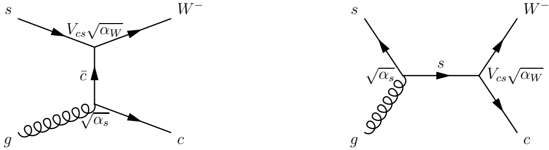
Figure 2.4: sg \rightarrow Wc Feynman diagrams.
