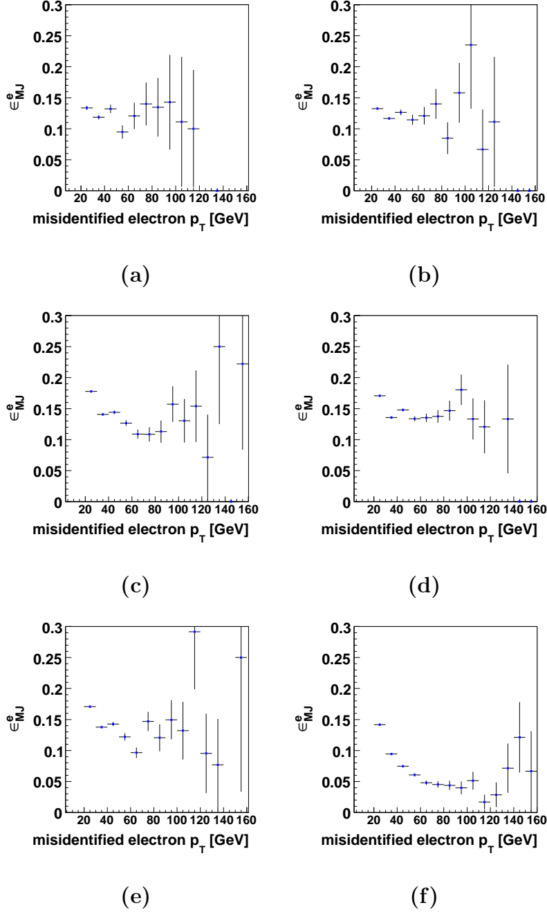
Figure 6.8: The electron mis-identification rate estimated from Jet-EM data sample as a function of p_T^e , (a) run range [ < 173101 ], (b) run range [173516-178721], (c) run range [178722-194568], (d) run range [194569-208122], (e) run range [208204-210711], (f) run range [ > 210835 ].
