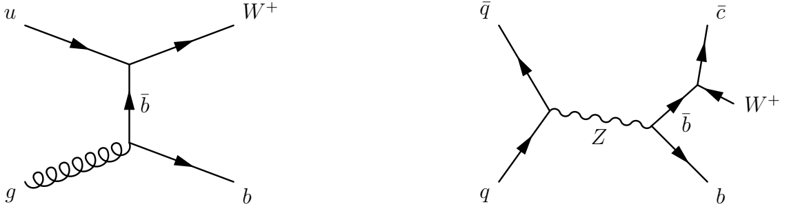
Figure 7.7: Possible diagrams for W + b and W + b\bar{c} processes. Contribution to these background processes is suppressed by small cross sections.
