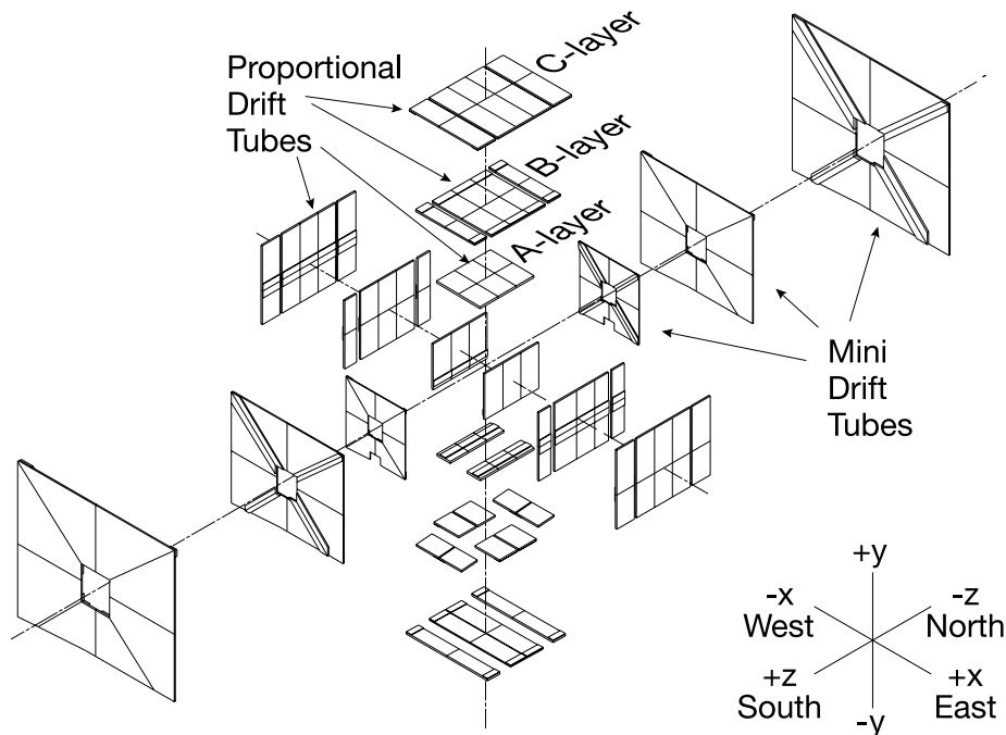
Figure 3.17: Schematic view of layers of drift chambers in D\phi muon system.
