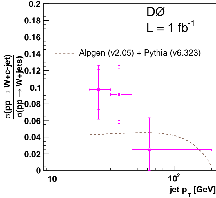
Figure 8.2: Combined measurement of the ratio \frac{\sigma(p\bar{p} \rightarrow W+c\text{-jet})}{\sigma(p\bar{p} \rightarrow W+\text{jets})} in the electron channel and the muon channel, for the particle level corrected p_T with a minimum threshold of 20 GeV and the pseudorapidity |\eta| < 2.0 in each p_T bin. The data points are shown with the theoretical expectation of ALPGEN+PYTHIA. Inner error bars represent the statistical only uncertainty on the measurement and the outer error bars corresponds to the total uncertainty where statistical and systematic uncertainties are added in quadrature.
