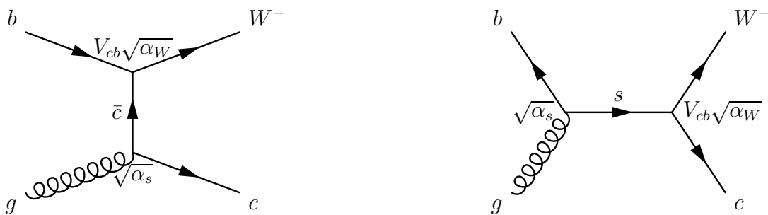
Figure 2.6: bg \rightarrow Wc Feynman diagrams.
