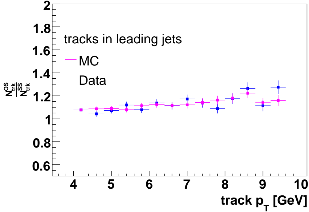
Figure 7.12: A comparison of data for the ratio of the OS weighted tracks to SS weighted tracks present in the leading jet with the ratio of the OS pions to SS pions present in the jet is shown as a function of track transverse momentum p_T .
