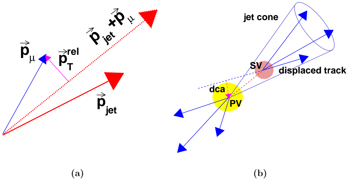
Figure 7.23: (a) The relative transverse momenta of the muon with the axis formed by the jet momentum direction and the muon momentum direction, p_T^{rel} , (b) Schematic diagram for the distance of closest approach (also called impact parameter) of the displaced track with respect to the primary vertex.
