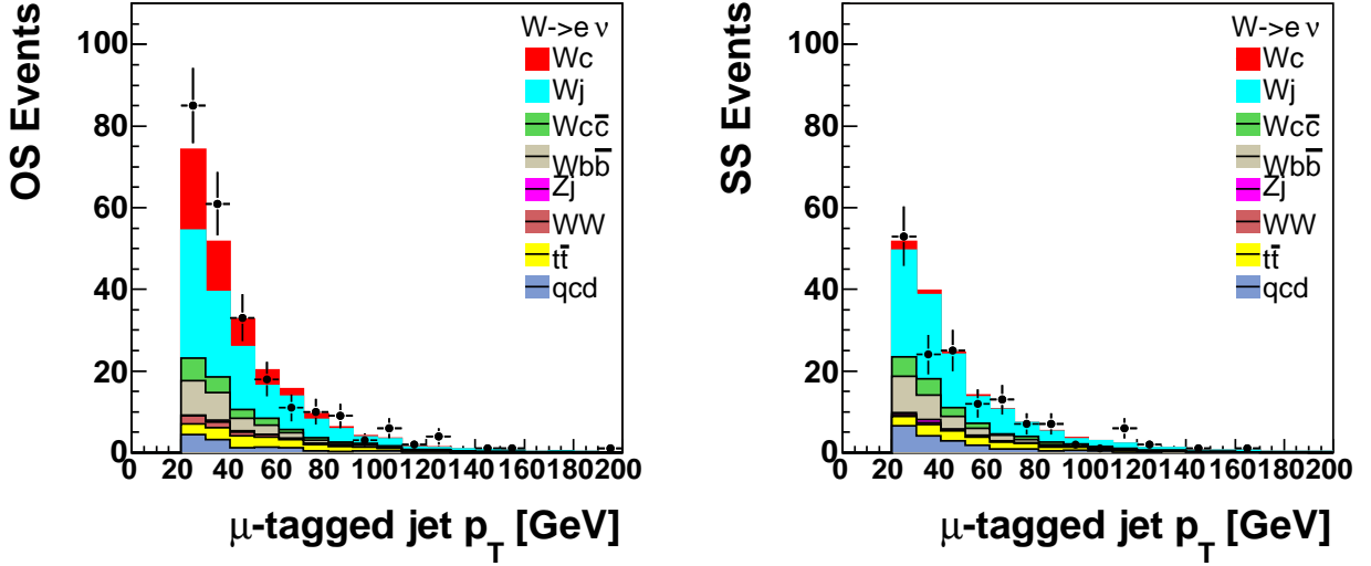
Figure 7.8: The jet p_T distribution of the \mu -tagged jet in the W(\rightarrow e\nu)+\mu -tagged jet sample after the final selection. Events with the isolated muon charge opposite (equal) to that of the muon present in the jet, OS events (SS events), are shown on the left (right) side. The total MC prediction is the sum of the expectations from the W + c -jet, W + light-jet, W + c\bar{c} , W + b\bar{b} , Z + jets, WW , t\bar{t} production processes estimated from ALPGEN-PYTHIA and the QCD jet production estimated from the data sample as described in Sec. 7.3.3.
