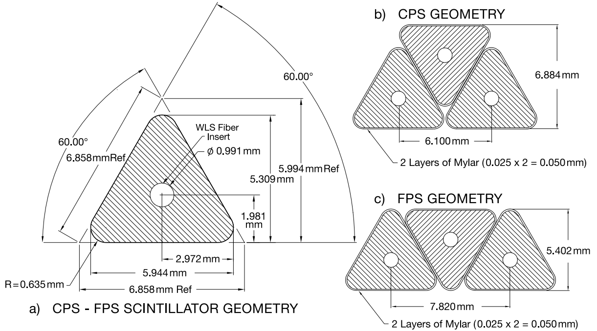
Figure 3.13: Schematic view of a unit preshower detector at D\bar{O} .
