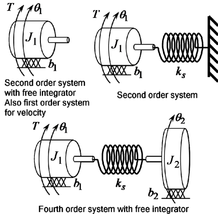
Fig. 3. Variations on the mechanical model
