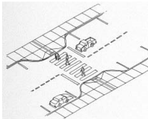
Figure 1.5: Curb Extensions and Highly Visible Crosswalks Improve Pedestrian Access at Mid-block Crossings
