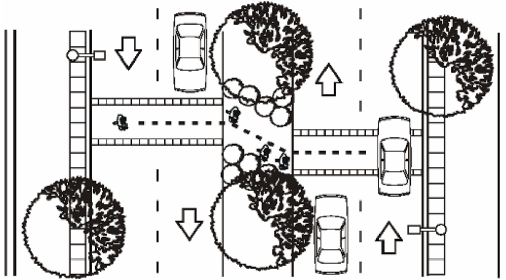
Figure 1.6: Staggered Crossing Configuration
