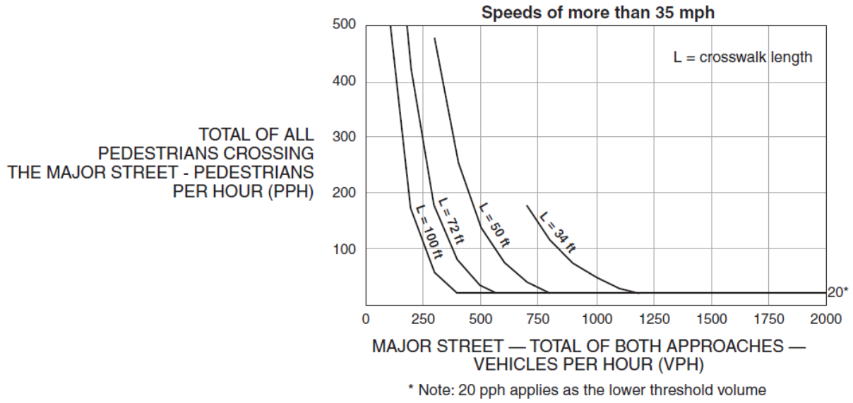
Figure 4.2: Guidance for Installation of Pedestrian Hybrid Beacons on High-Speed Roadways
