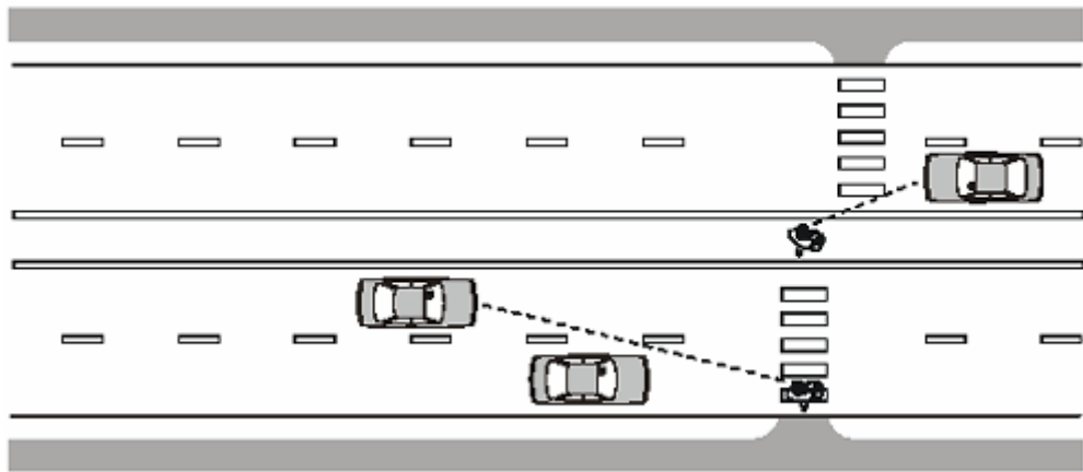
Figure 1.3: Mid-block with Median Refuge Allows the Pedestrian to Look for Gaps in Only One Direction at a Time
