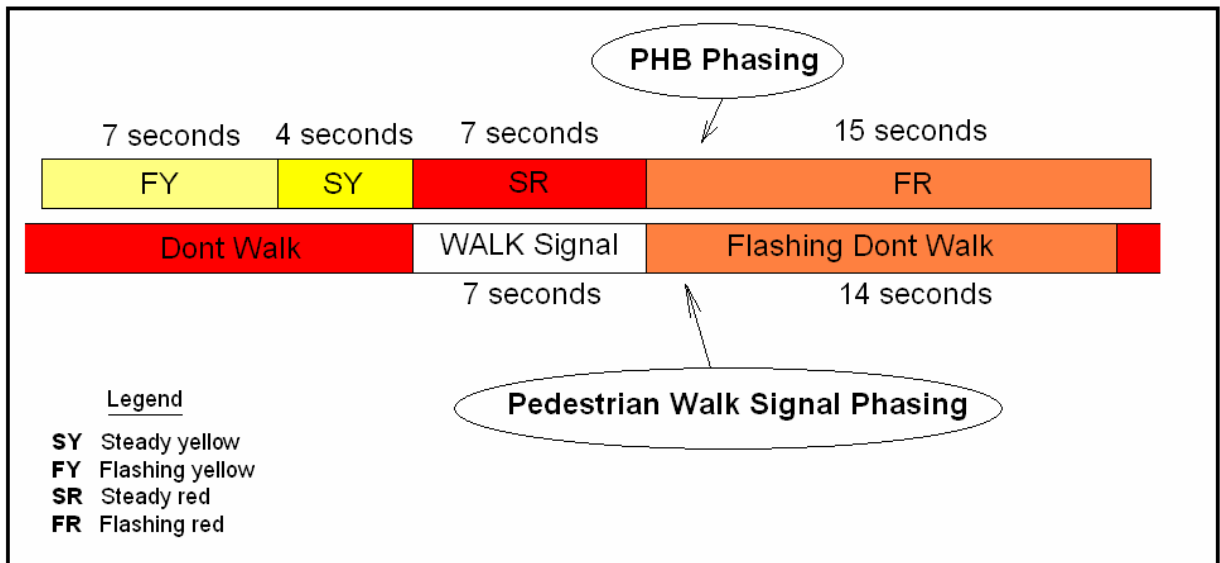
Figure 5.2: Designed Signal Timings for Pedestrian Hybrid Beacon Coordinating with Pedestrian Walk Signals on 11th Street, Lawrence, Kansas
