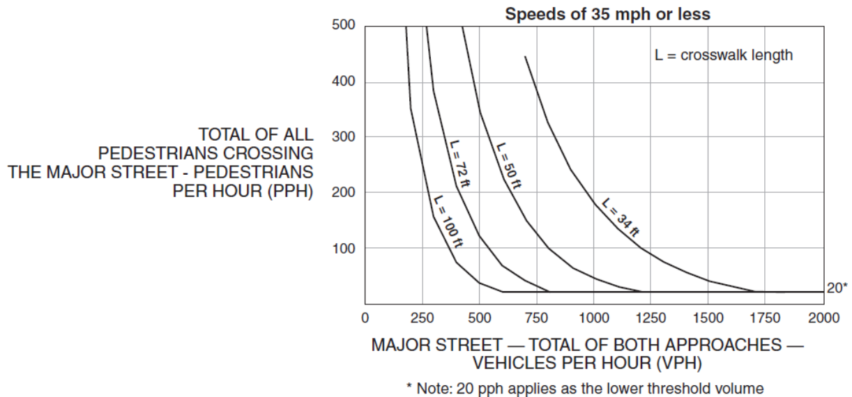
Figure 4.1: Guidance for the Installation of Pedestrian Hybrid Beacons on Low Speed Roadways
