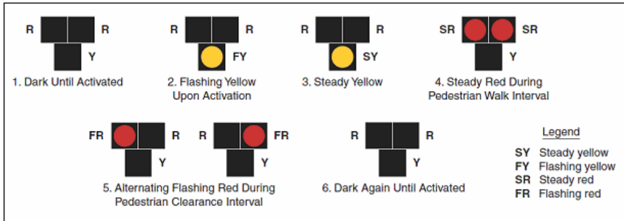
Figure 1.8: Sequence of Operation for a Pedestrian Hybrid Beacon
