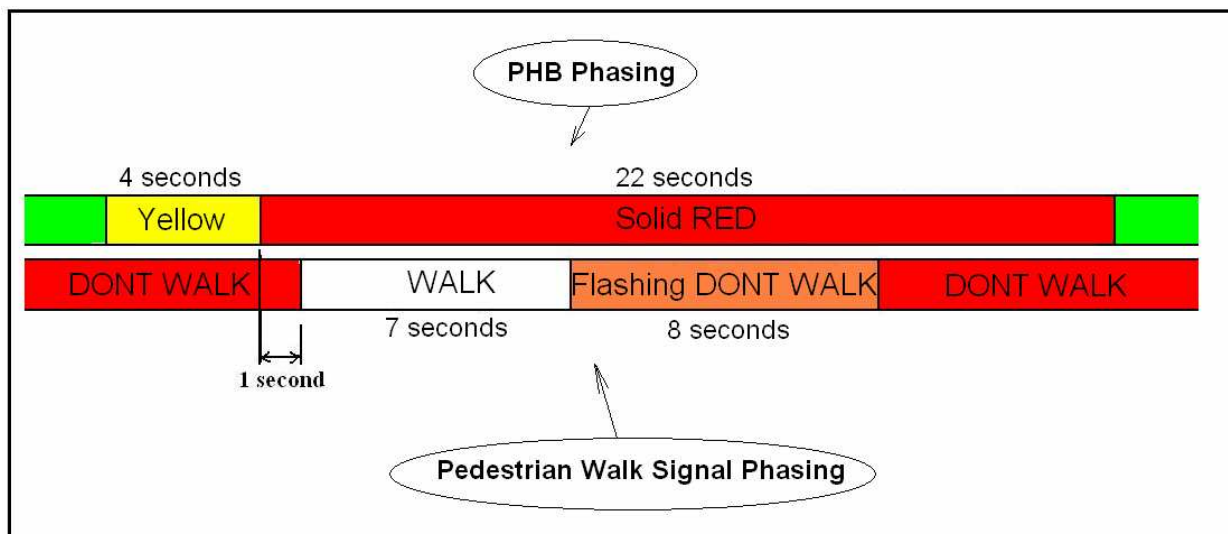
Figure 5.6: Designed Signal Phasing Times for Signalized Mid-block Coordinating with Pedestrian Walk Signals on Massachusetts Street
