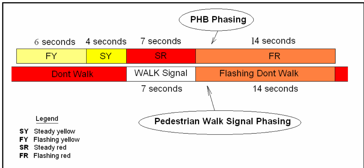
Figure 5.4: Designed Signal Timings for Pedestrian Hybrid Beacon Coordinating with Pedestrian Walk Signals on New Hampshire Street.
