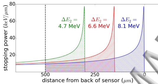
FIG. 3. Bragg curves for protons stopping at different locations within a 500 \mu\text{m} monolithic silicon sensor. The integral over the deposited energy in the sensor, \Delta E_2 , and consequently, the calculated dE/dx depends on the depth reached by the proton before stopping.
