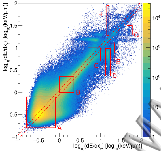
(a) dE/dx_1 vs. dE/dx_2 for data acquired on ISS outside of the SAA region with highlighted areas of interest.
