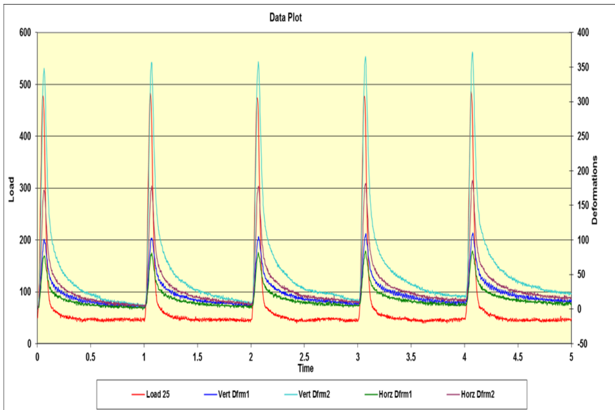
Figure 4.4 Typical output of resilient modulus from IDT test software
