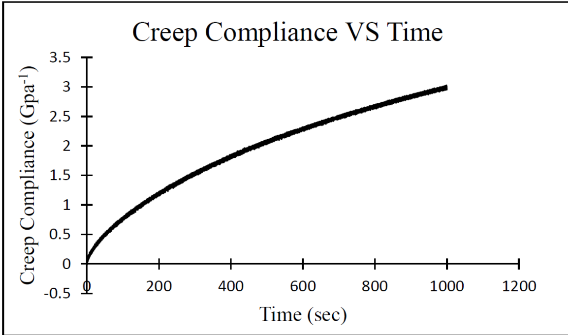
Figure 2.4 Typical creep compliance test output (Gong, et al., 2012)
