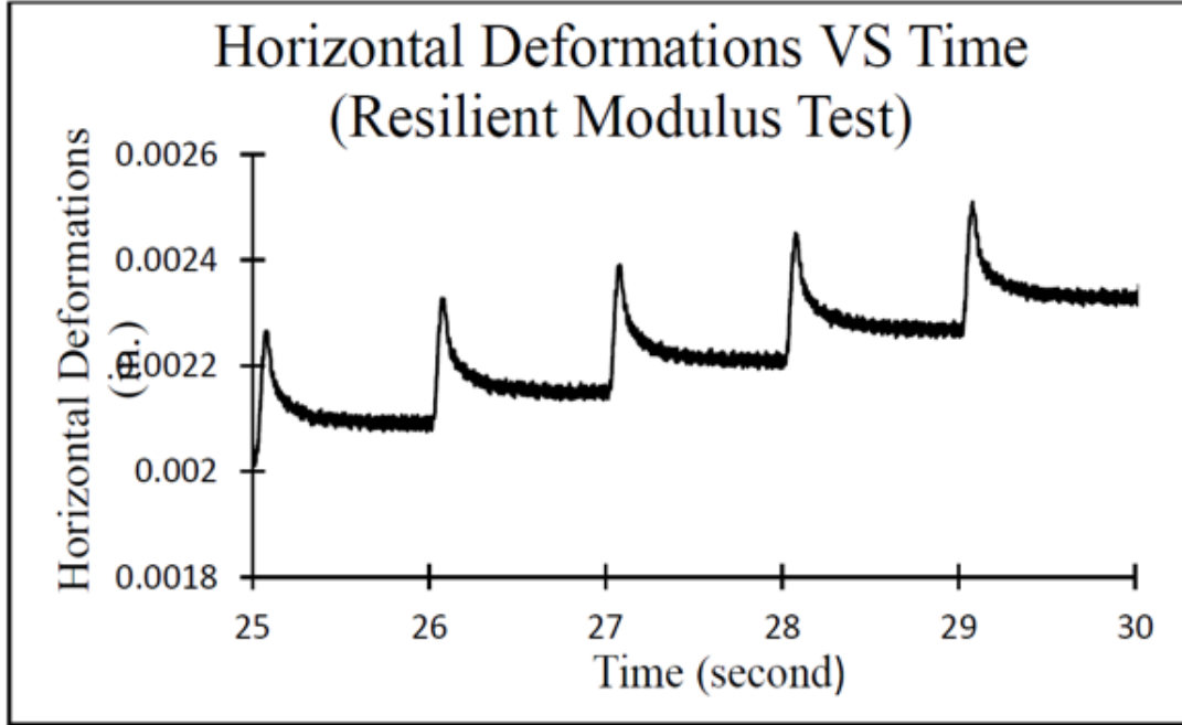
Figure 2.3 Typical resilient modulus test output (Gong, et al., 2012)
