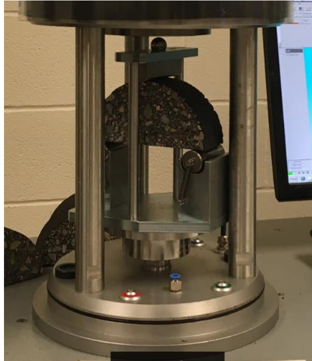
Figure 3.4 SCB test setup
