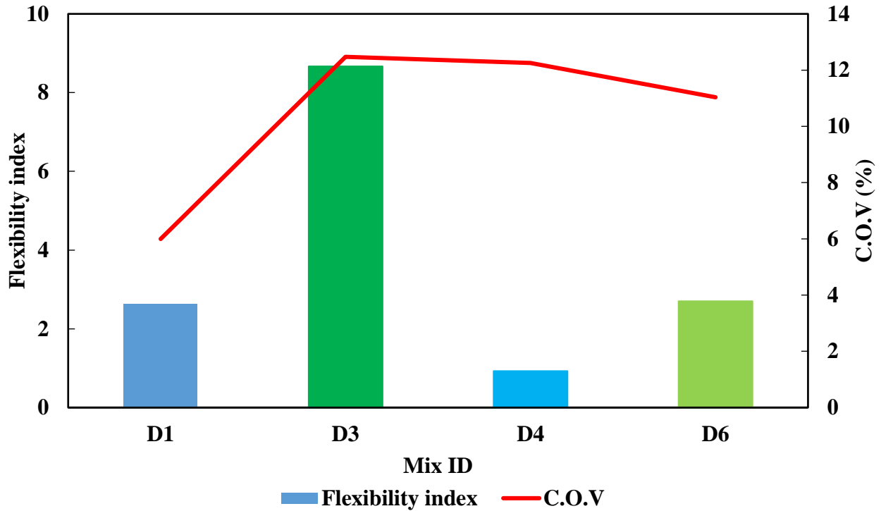
Figure 4.3 Test results of FI and COV
