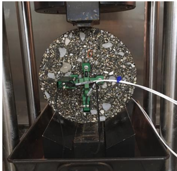
Figure 3.5 IDT rest setup
