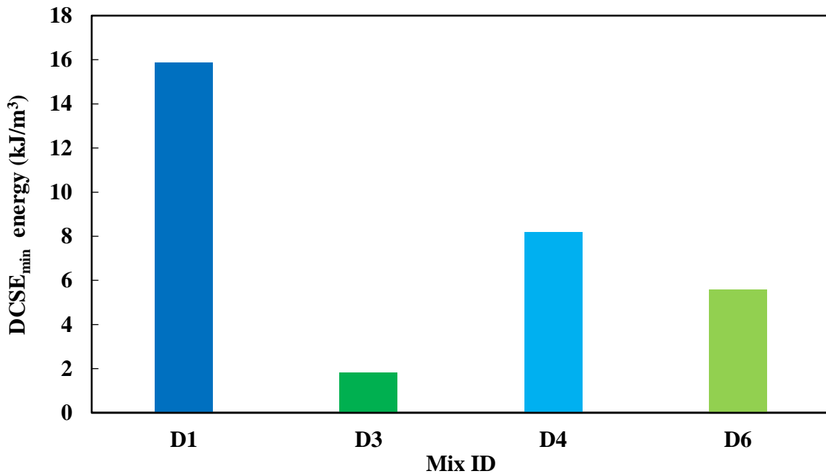
Figure 4.11 DCSE min results
