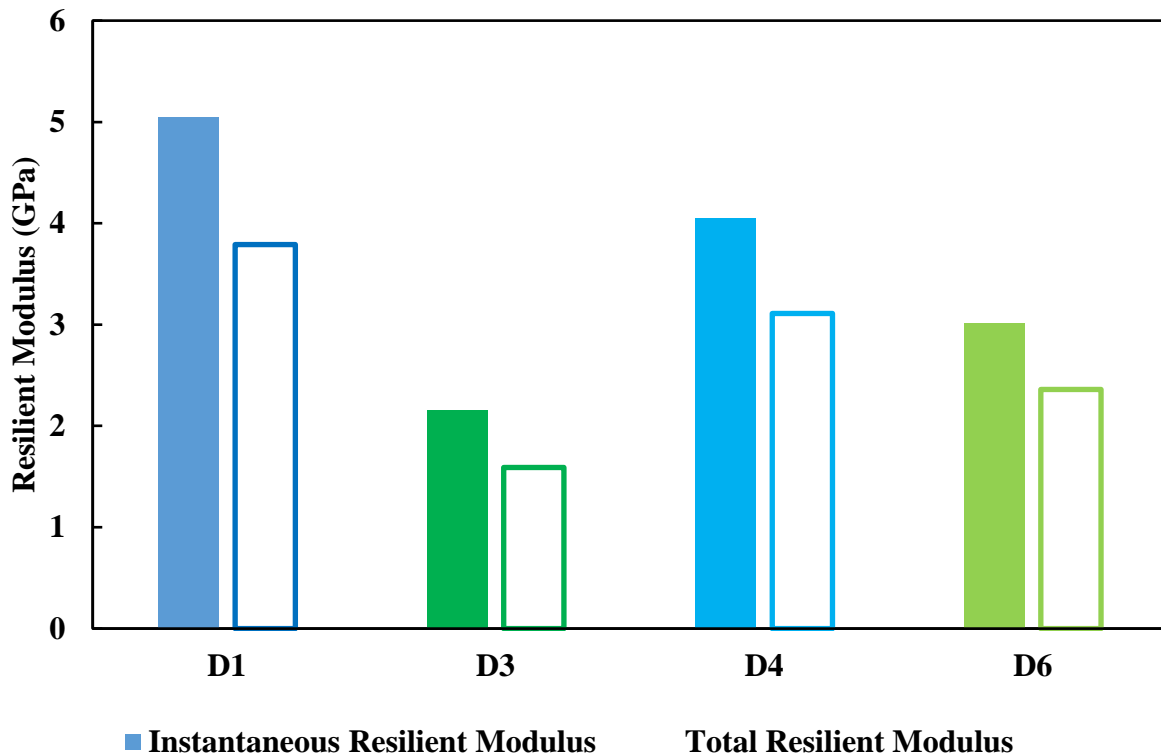
Figure 4.5 Resilient modulus test results
