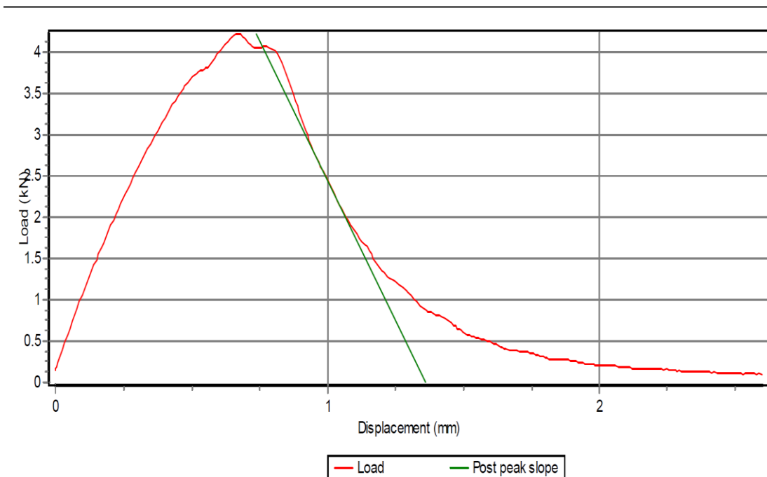
Figure 4.1 Typical output from SCB test software
