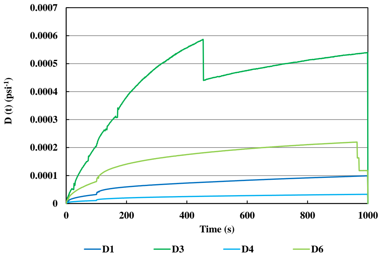
Figure 4.6 Creep compliance curve
