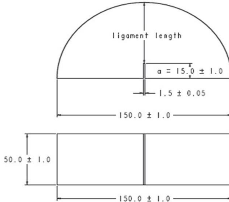
Figure 2.1 SCB test specimen configuration (AASHTO TP 124, 2016)
