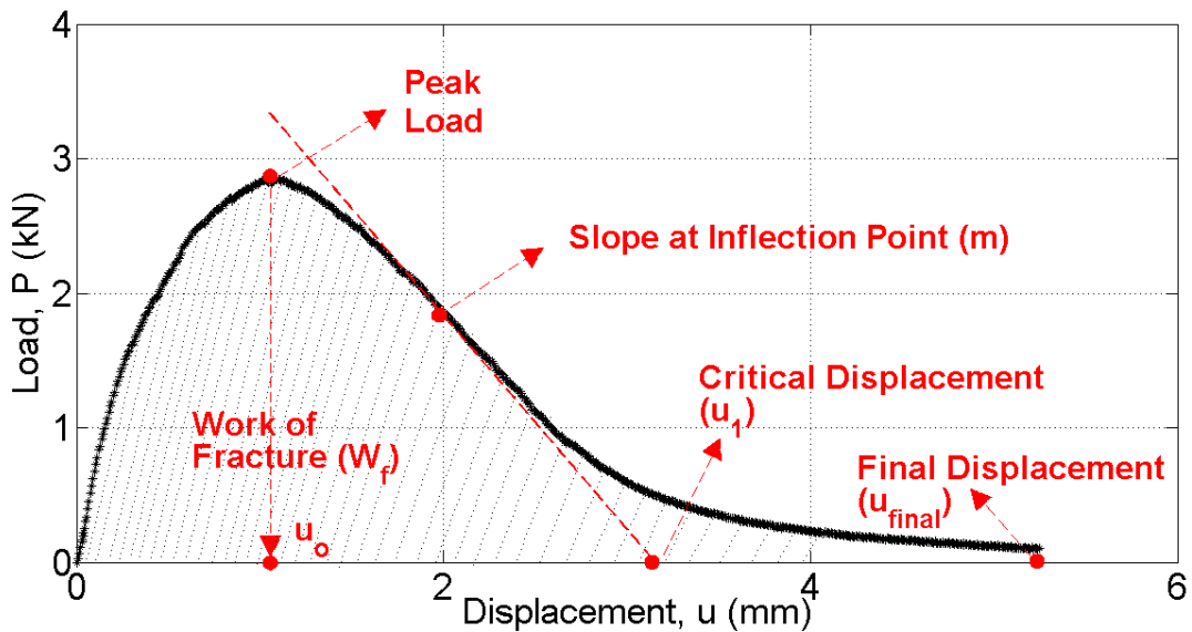
Figure 2.2 Recorded load versus load-line displacement curve (AASHTO TP 124, 2016)
