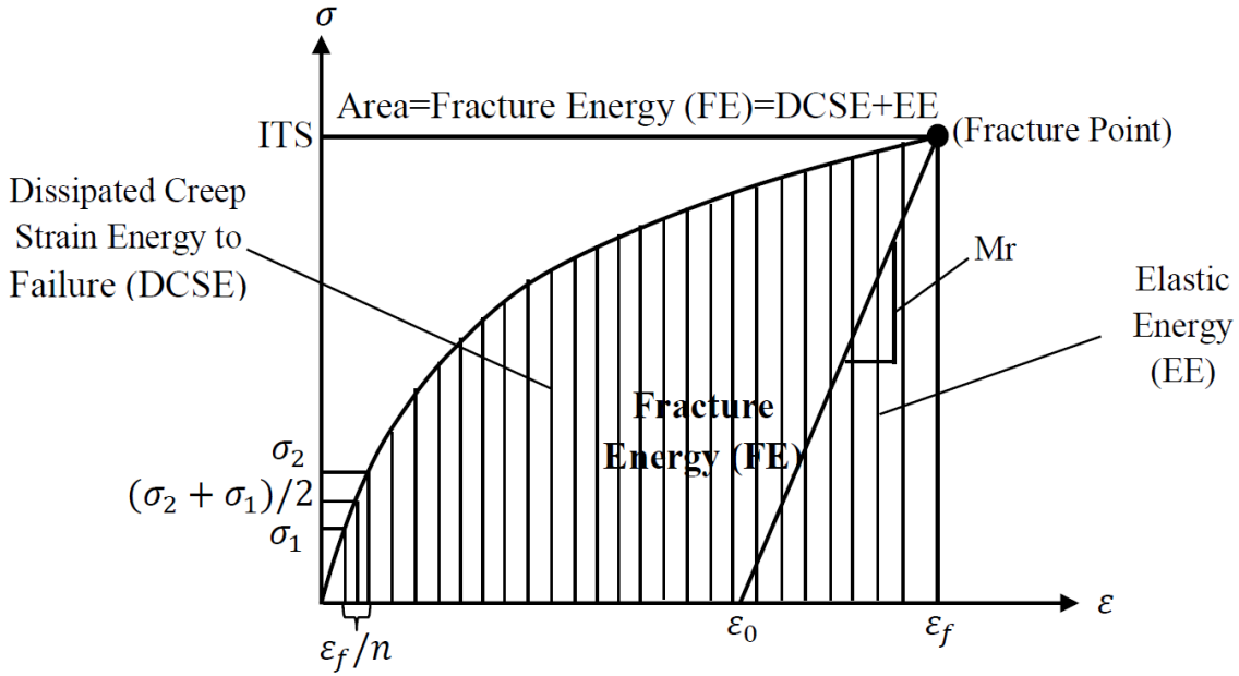
Figure 2.5 Relationship between FE, EE, and DCSE f (Gong, et al., 2012)
