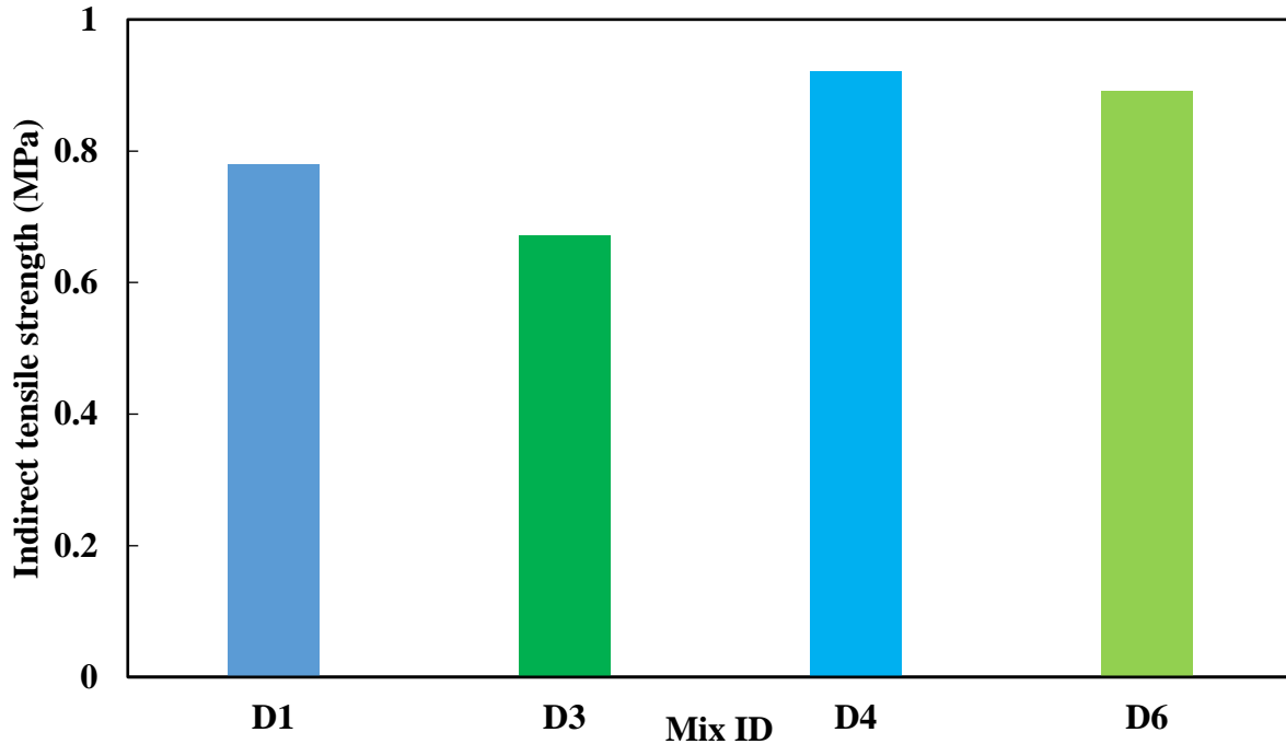
Figure 4.7 IDT test results
