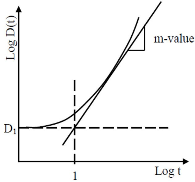
Figure 2.6 Creep compliance curve in logical coordinates (Gong, et al., 2012)
