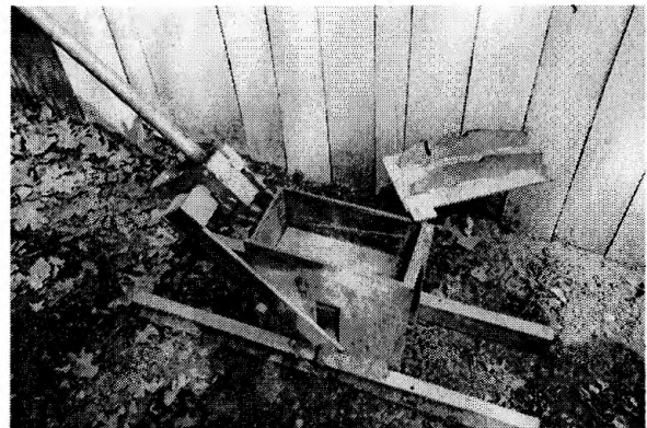
FIG. 23 STATICALLY COMPACTED MOULD
