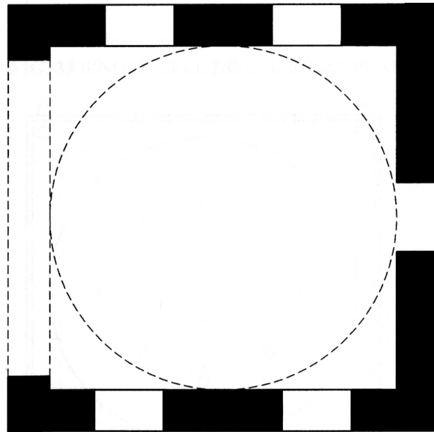
FIG. 32 SINGLE CELL STRUCTURAL PLAN
