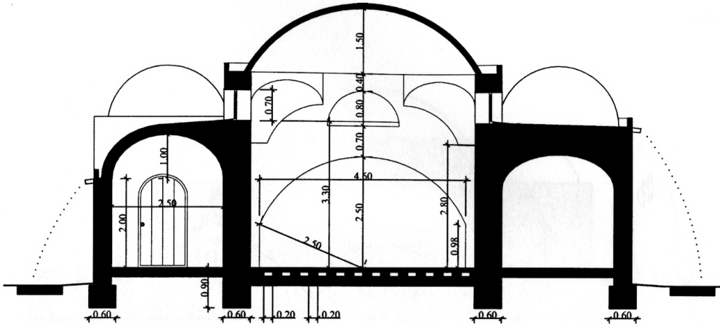
FIG. 48 SINGLE UNIT A-A SECTION
