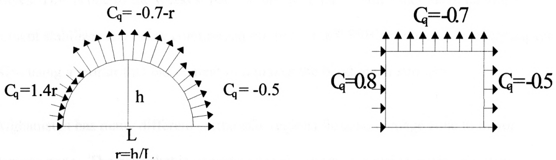
FIG. 90 C q FOR DOME SHAPES
