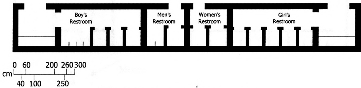
FIG. 67 RESTROOM UNITS PLAN
