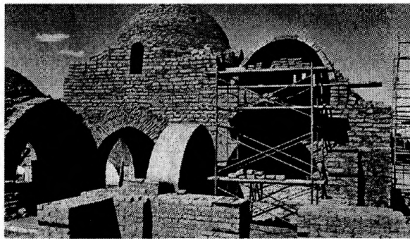
FIG. 4 ADOBE BRICK CONSTRUCTION
