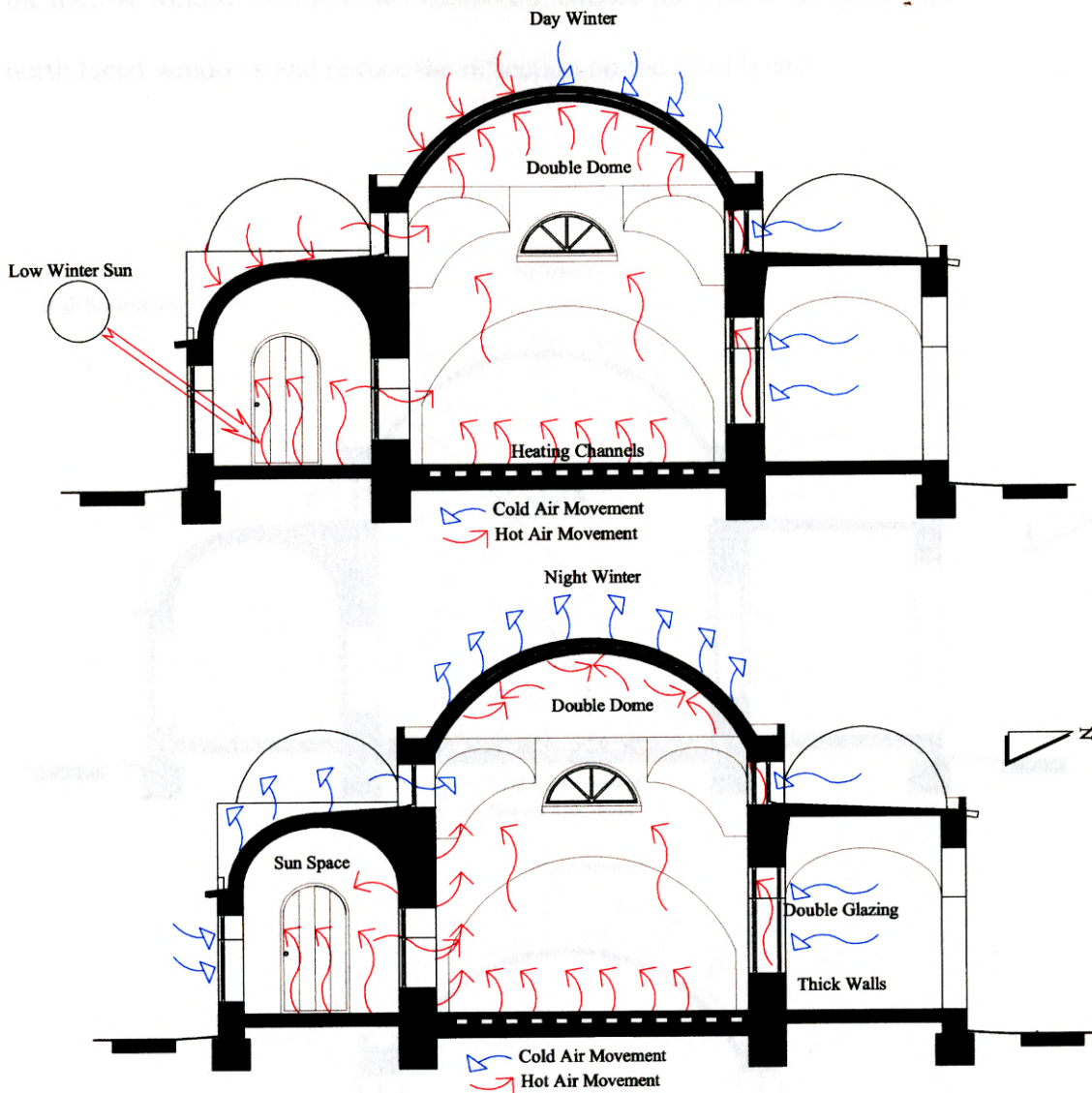
FIG. 27 PASSIVE & ACTIVE HEATING
