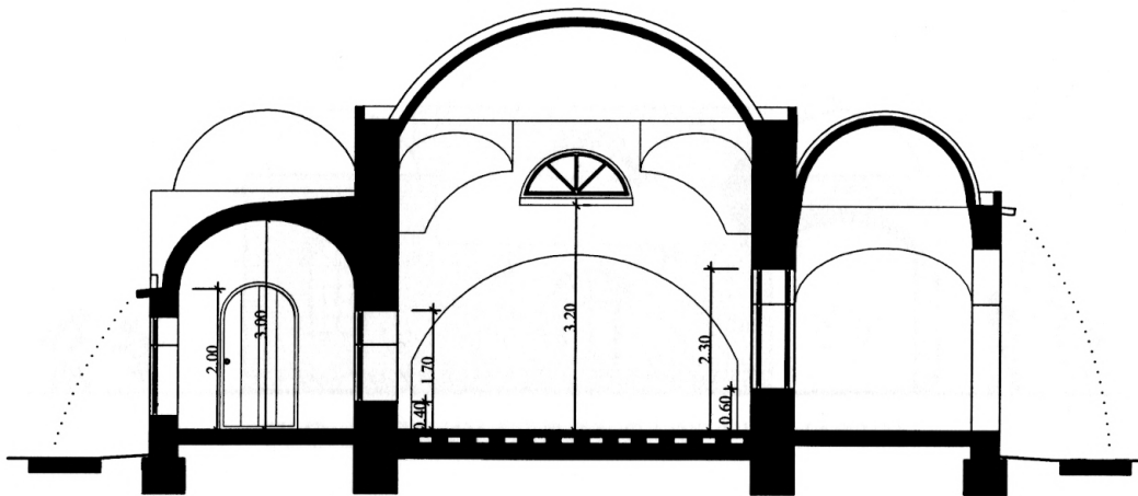
FIG. 49 SINGLE UNIT B-B SECTION
