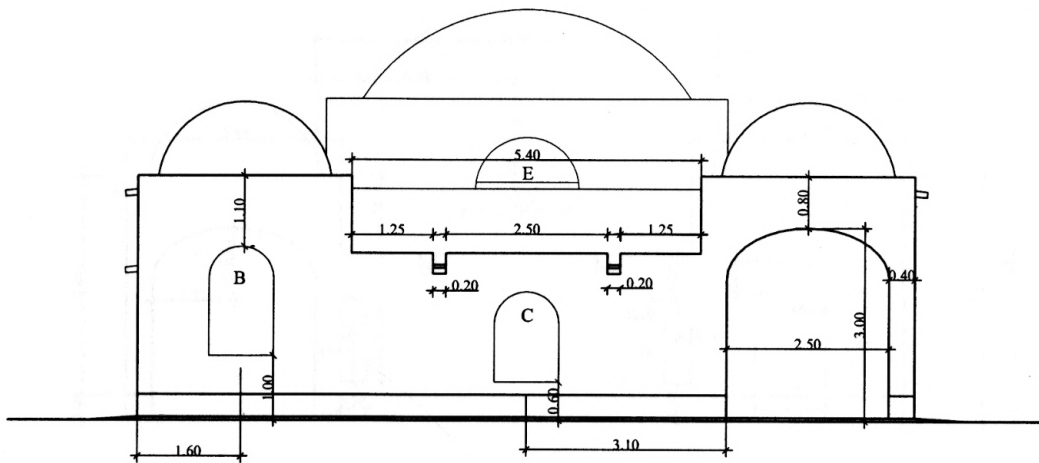
FIG. 55 SINGLE UNIT DIMENSIONAL EAST ELEVATION
