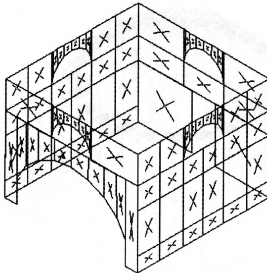
FIG. 83 WIRE FRAME OF THE WALLS
