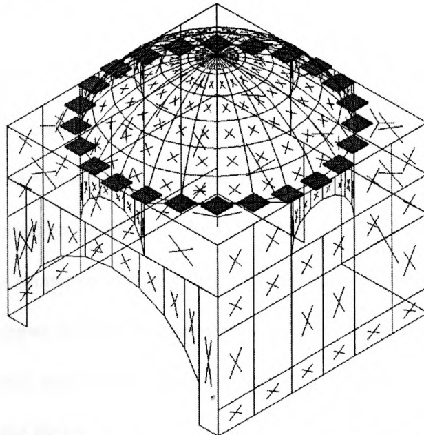
FIG. 85 RIGID LINKS BETWEEN THE DOME AND THE WALLS
