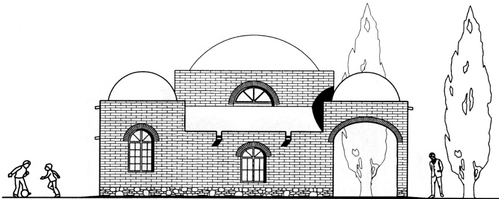
FIG. 51 SINGLE UNIT EAST ELEVATION
