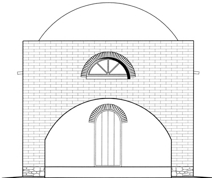
FIG. 38 SINGLE CELL WEST ELEVATION
