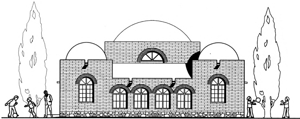
FIG. 50 SINGLE UNIT SOUTH ELAVATION
