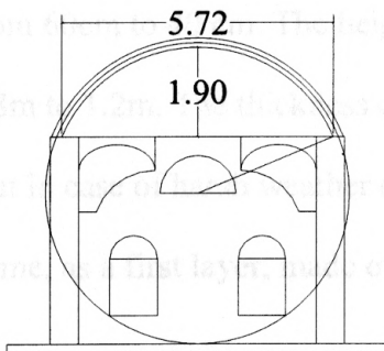
FIG. 92 CASE STUDY MODELS: PROPORTION OF HEIGHT TO BREADTH OF THE DOME
