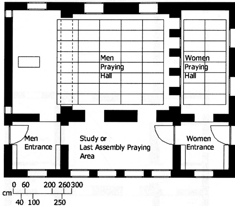
FIG. 62 MOSQUE PLAN
