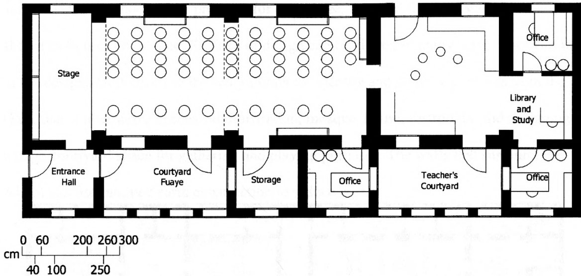
FIG. 66 ADMINISTRATIVE UNIT PLAN
