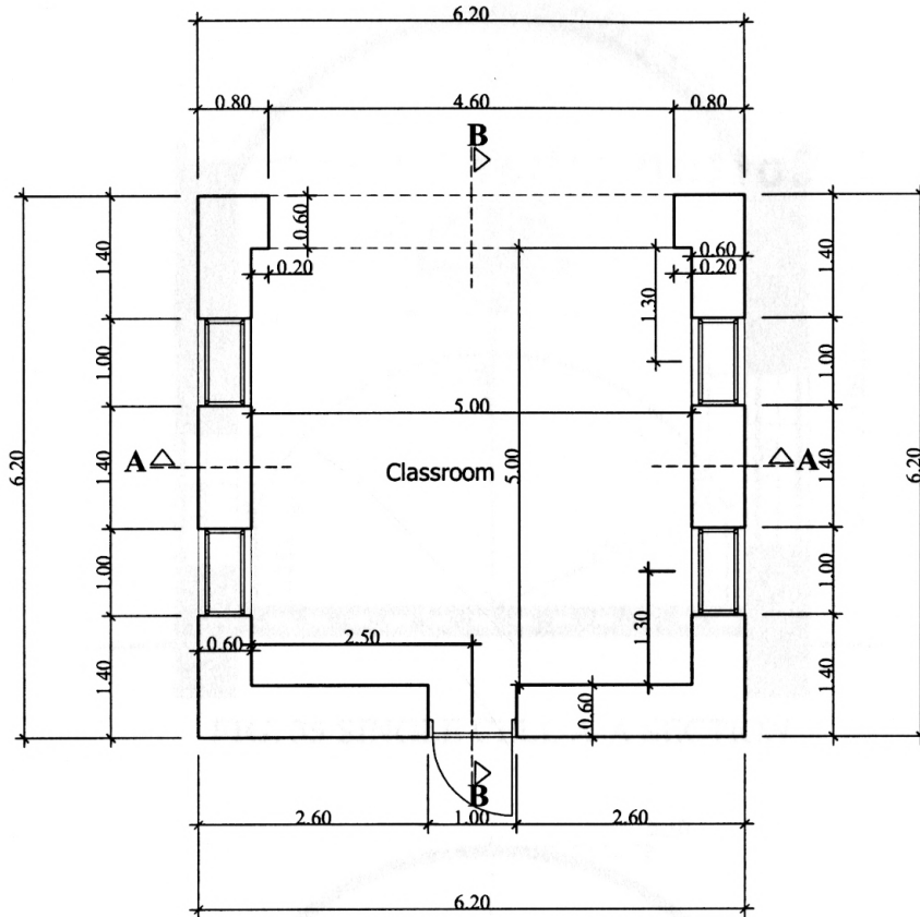
FIG. 33 SINGLE CELL DIMENSIONAL PLAN
