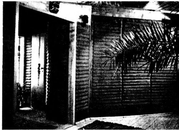
FIG. 8 STRANGLEHM TYPE OF CONSTRUCTION
