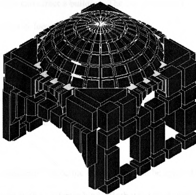
FIG. 86 COMPLETED MODEL, 80% RENDERED
