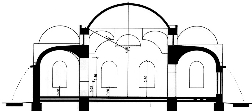
FIG. 47 SINGLE UNIT C-C SECTION
