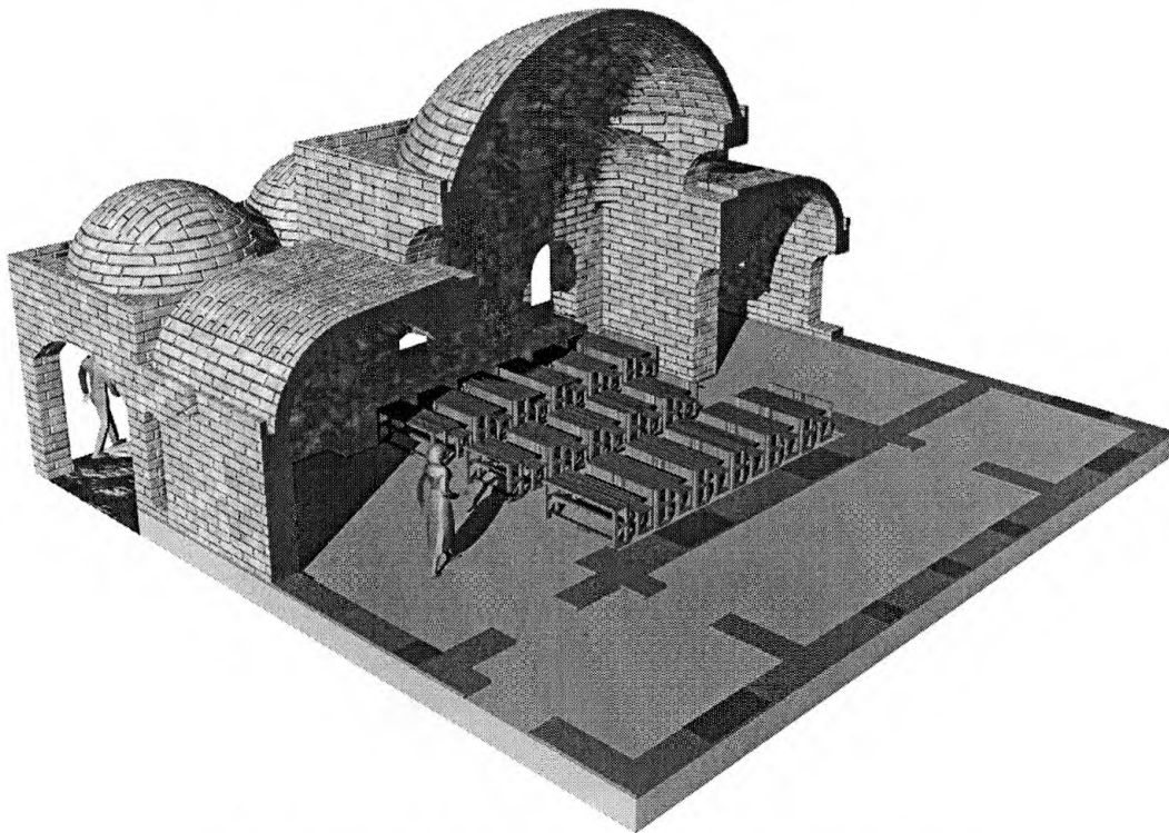
FIG. 60 SINGLE UNIT RENDERED SECTION C-C
