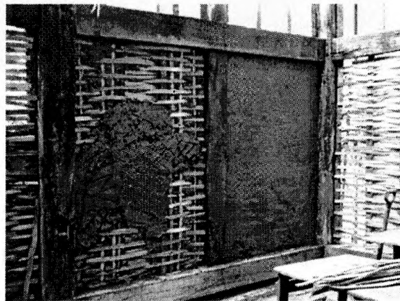
FIG. 6 WATTLE AND DAUB CONSTRUCTION
