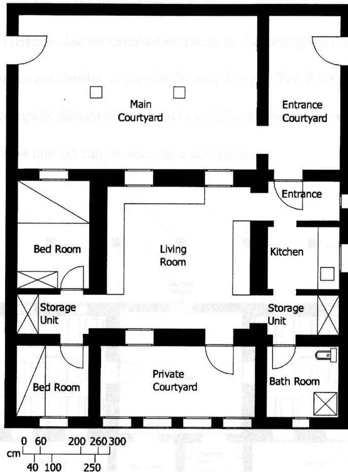
FIG. 63 HOUSE PLAN
