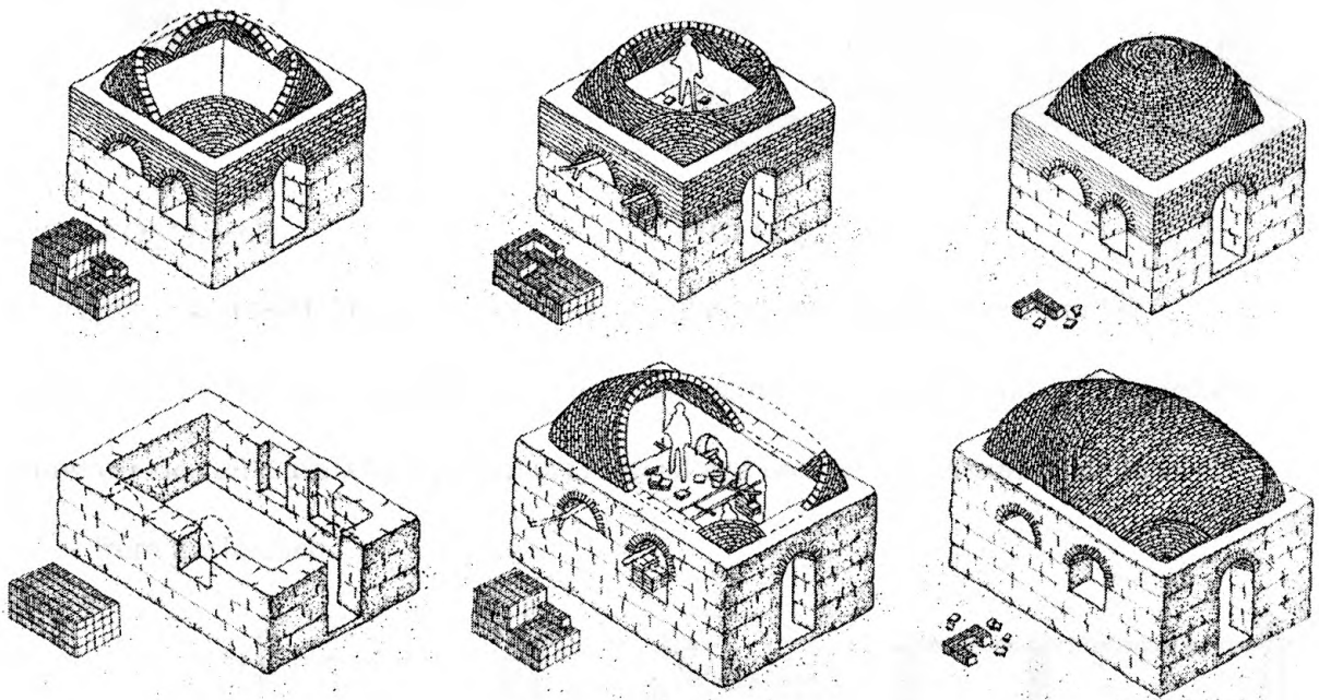
FIG. 11 TRADITIONAL AFGHAN VAULTING METHOD
