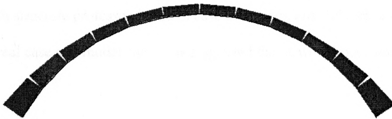
FIG. 71 SHALLOW VAULT, PREVIOUSLY DESIGNED MODEL
