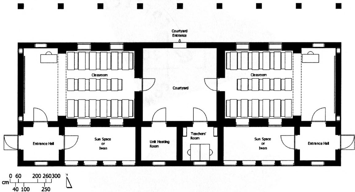
FIG. 64 DOUBLE UNIT SCHOOL PLAN
