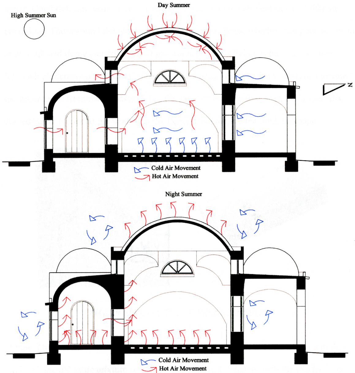
FIG. 28 PASSIVE COOLING
