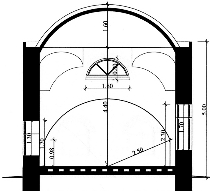
FIG. 35 SINGLE CELL A-A SECTION
