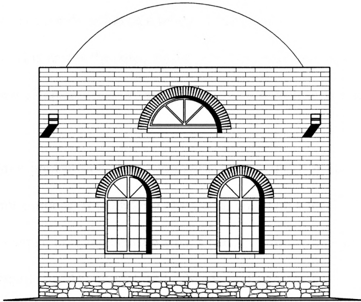
FIG. 39 SINGLE CELL NORTH ELEVATION
