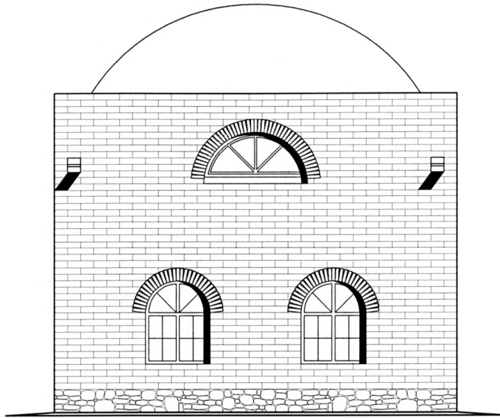
FIG. 37 SINGLE CELL SOUTH ELEVATION
