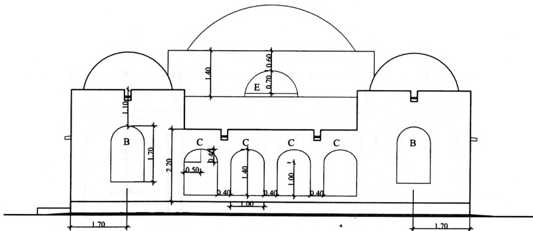
FIG. 54 SINGLE UNIT DIMENSIONAL SOUTH ELEVATION
