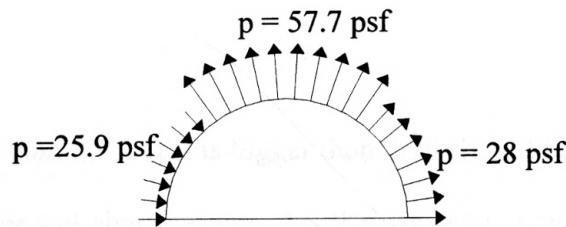
FIG. 91 WIND LOAD ACCORDING TO THE SHAPE OF THE DOME
