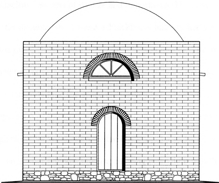
FIG. 40 SINGLE CELL EAST ELEVATION
