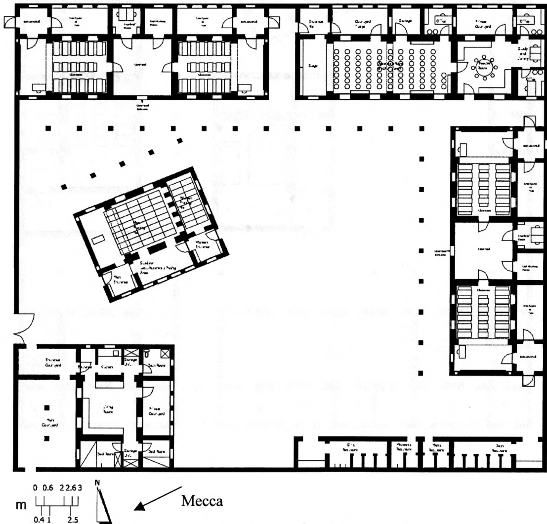
FIG. 68 FOUR UNIT SCHOOL PLAN
