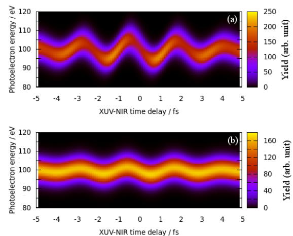
Figure 2. Calculated streaking spectra from a single initial state of a spherical square well potential (at the Fermi level with zero angular momentum) representing a 10 nm diameter gold nanosphere. (a) With plasmonically enhanced near field and (b) without near field enhancement.
