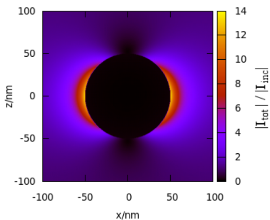
Figure 1. Total field enhancement near a 100 nm diameter gold nanosphere at x-z plane, driven by a 800 nm plane wave propagating in z-direction and polarized in x-direction. Maximum enhancement is found along polarization direction.
