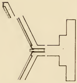
SECTION THROUGH THE REINFORCED CONCRETE WALL
