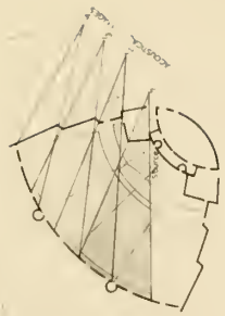
AUDITORIUM SHAPING POSITION OF SOME REINFORCEMENT PLATES
