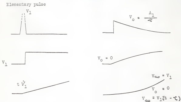
Fig. 16. Output of a low pass filter to inputs of elementary pulses.
