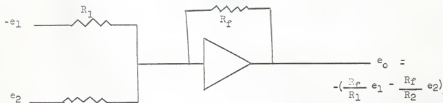
Fig. 4. Subtraction on an operational amplifier.
