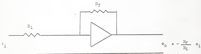
Fig. 2. Operational amplifier for scalar multiplication operation, with ground connection shown.
