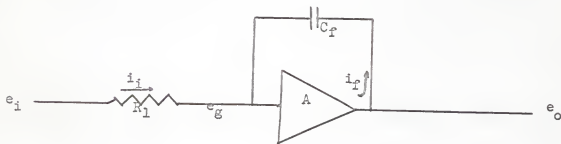
Fig. 6. Integration on an operational amplifier.
