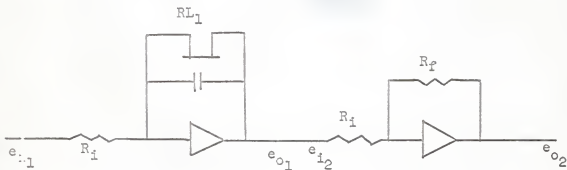
Fig. 23. Instant replenishment model
