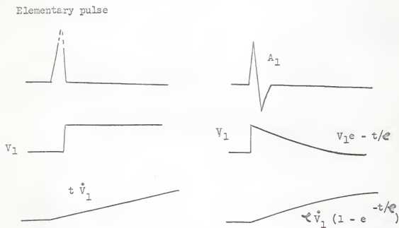
Fig. 17. Output of high pass filter to elementary pulse inputs.
