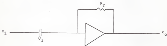
Fig. 5. Differentiation on an operational amplifier.
