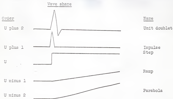
Fig. 13. Transient orders of elementary pulses.
