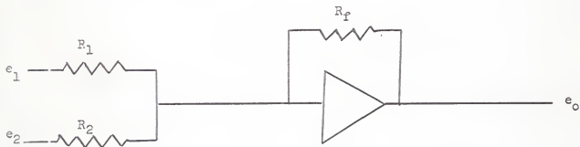
Fig. 3. Operational amplifier for addition; ground circuit omitted.
