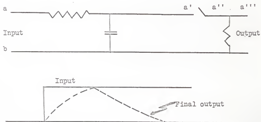
Fig. 20. Low pass filter with an output resistance representing finite replenishment and demand.
