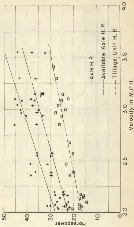
Fig. 8. The axle, available axle, and the tillage unit required horsepower versus speed curves for the clay soil.
