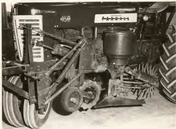
Fig. 1. The tillage unit of the I. H. C. 450 - 21 till-planter.
