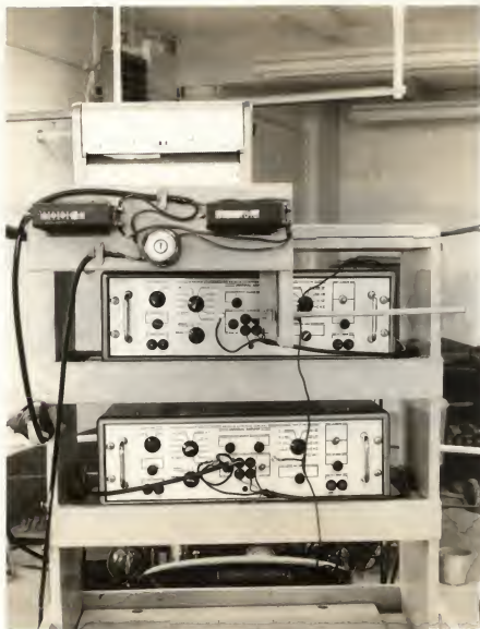
Fig. 7. The plywood instrument cabinet and the instruments used in the power requirement tests.
