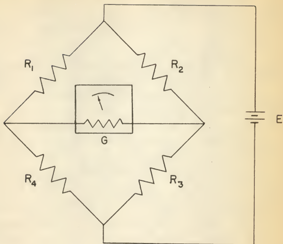
Fig. 2. The basic Wheatstone bridge circuit.
