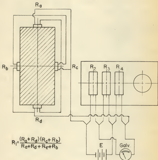
Fig. 4. Schematic wiring diagram of the bridge circuit used in measuring tillage unit draft with R_1 , R_2 , R_3 , and R_4 located within the bridge as they were in Fig. 2.
