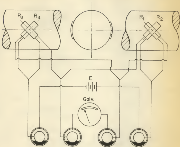
Fig. 3. Schematic wiring diagram of the bridge circuit utilized in measuring axle torque with R_1 , R_2 , R_3 , and R_4 located the same within the bridge as they were in Fig. 2.
