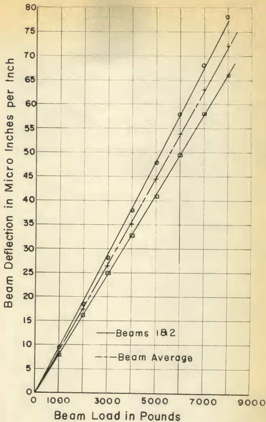
Fig. 5. Micro-inches of deflection versus tillage unit beam load in pounds.
