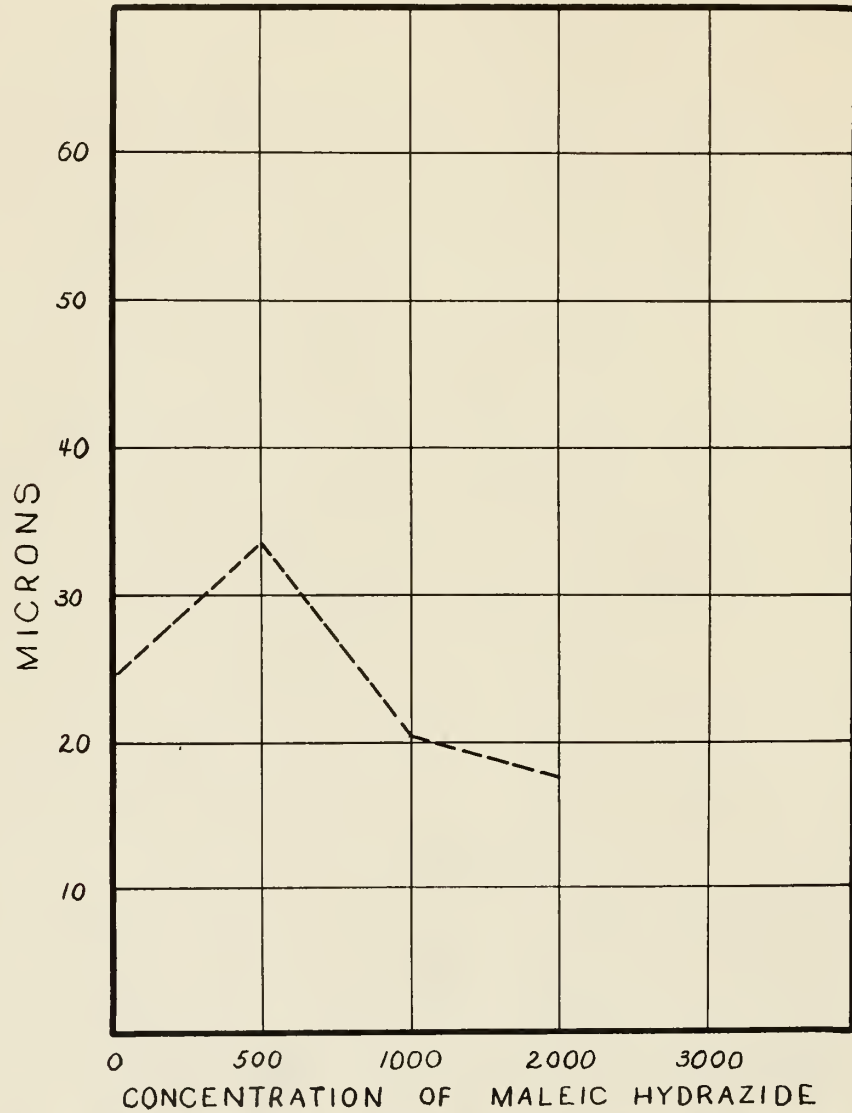
Fig. 7. The depth of the palisade cells of raspberry leaves as influenced by the application of maleic hydrazide. The initial readings represents the depth of the palisade cells of the untreated leaves.
