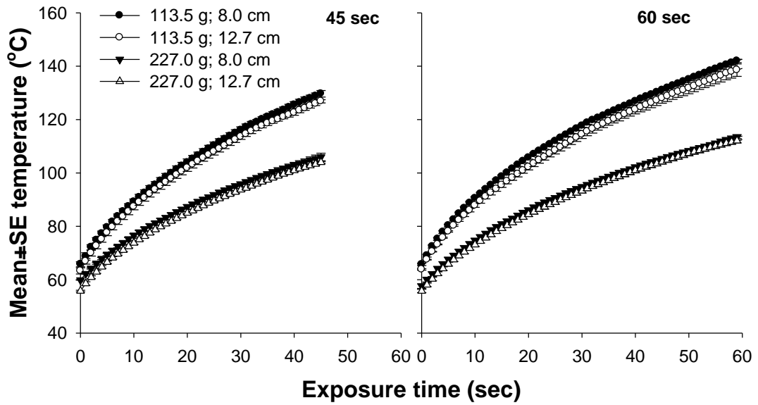
Figure 4:1. A generalized time-dependent temperature profile attained with different quantities of wheat exposed at 8.0 and 12.7 cm from the emitter for 45 or 60 sec.
