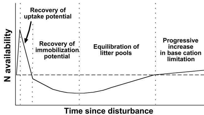
Fig. 3. Conceptual diagram of N availability for northern hardwood forests during secondary succession. N availability rises with disturbance, but the recovery of vegetation uptake potential generally decreases N availability soon after. N availability can continue to decline, potentially even below predisturbance N availability, if soil and litter fractions were depleted by disturbance and their recovery immobilizes N. The recovery of immobilization might be followed by an increase in N availability as these pools equilibrate, but there has been little research on these long-term dynamics. Over longer time scales, N availability increases with ecosystem development and increasing base cation limitation. Axes are not to scale.
