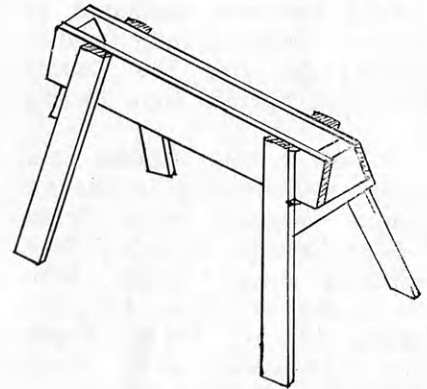
Open-Top Sawhorse
