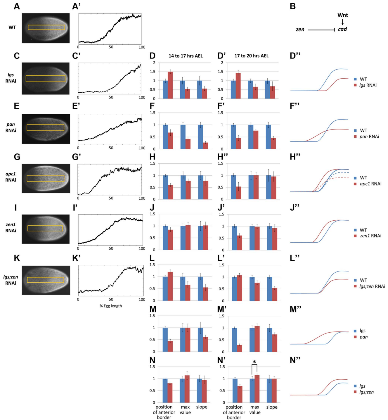
Figure 2. Characterization of Tc-cad gradient in WT and RNAi knockdowns. (A, A') Tc-cad gradient in WT. (B) A model for Tc-cad regulation in the Tribolium blastoderm. (C–D') Tc-cad gradient expression in a Tc-lgs RNAi embryo (C, C'), and the average of its three descriptors normalized to WT values (Text S3) in 14–17 AEL (D) and 17–20 AEL (D'). As inferred from (D, D'), a comparison between the spatial distribution of Tc-cad gradient in Tc-lgs RNAi embryos and that of WT is summarized in D' (not to scale). The same was performed for Tc-pan (E–F'), Tc-apc1 (G–H'; in H': dashed curve for 14–17 AEL and solid curve for 17–20 AEL), Tc-zen1 (I–J'), and Tc-lgs;Tc-zen1 (K–L') RNAi embryos. (M–M') the average of the three descriptors of the Tc-cad expression gradient in Tc-pan RNAi normalized to Tc-lgs RNAi values (Text S3). (N–N') the average of the three descriptors of the Tc-cad expression gradient in Tc-lgs;Tc-zen1 RNAi normalized to Tc-lgs RNAi values. Asterisk (*) represents p -value < 0.05. Anterior to the left. Error bars represent 95% confidence intervals. doi:10.1371/journal.pgen.1004677.g002
