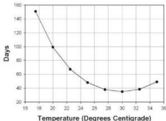
Figure 1. This shows egg-to-adult development time in days, as a function of temperature. As temperatures decrease, development time increases. Indian meal moth life stages also are impacted when temperatures rise above 35 degrees Centigrade.
