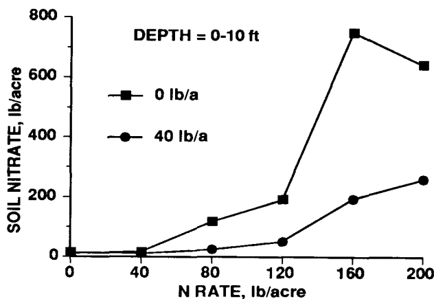
Figure 4. Effect of 30 years of N and P application to irrigated grain sorghum on NO 3 -N content of the soil profile (0 to 10 ft), Tribune, KS.
