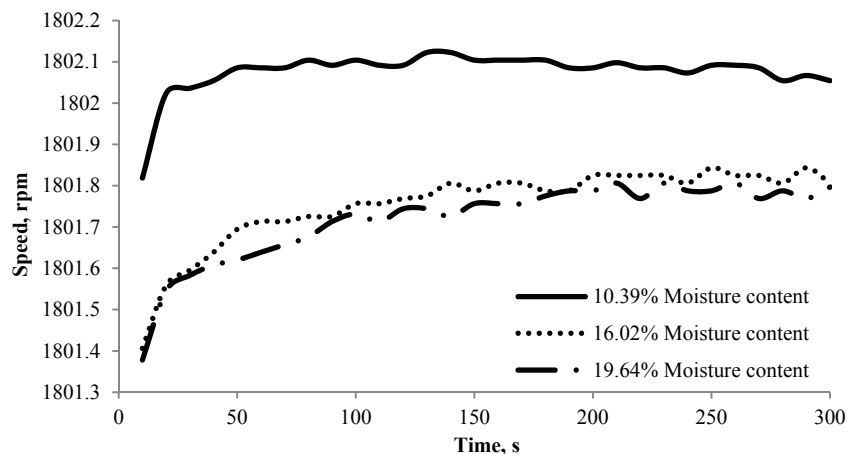
Figure 1. Hammermill rotor shaft speed during grinding of corn.
