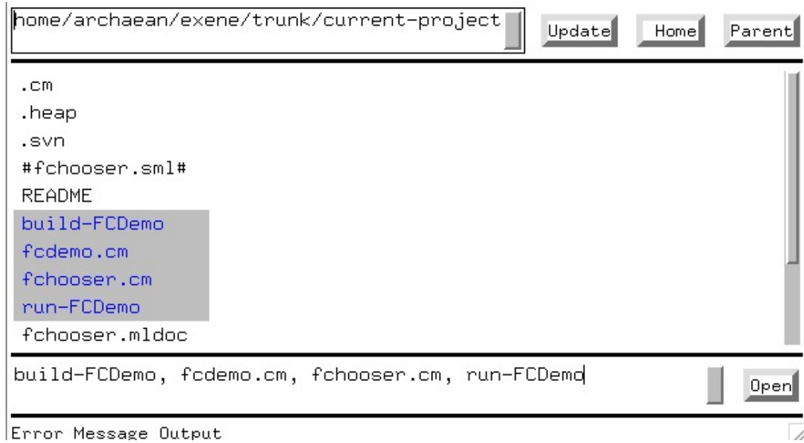
Figure 4.1: eXene file chooser screen shot
