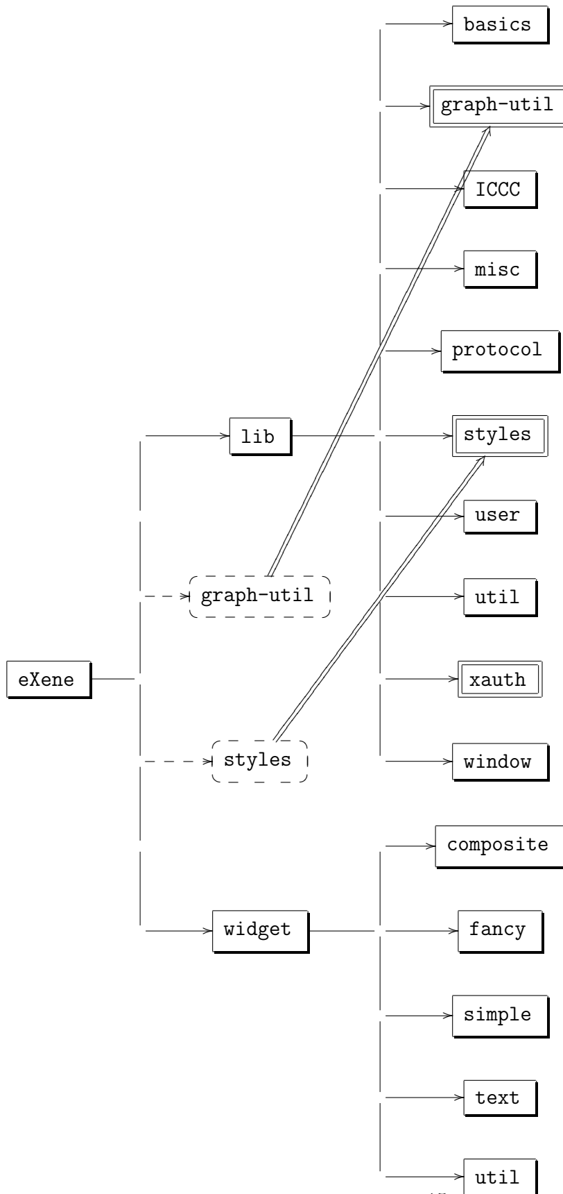
Figure 2.4: eXene directory refactorization
