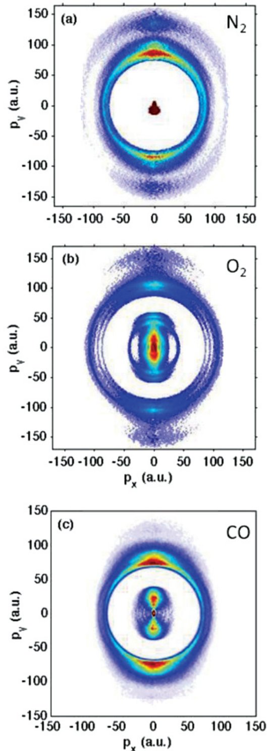
FIG. 1. (Color online) Inverted momentum images for detected (top to bottom) (a) N^+ , (b) O^+ , and (c) C^+ ions from N_2 , O_2 , and CO , respectively at the pump-probe delay of 500 fs.
