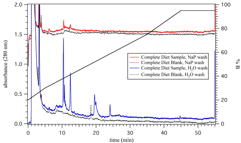
Figure 3.10: RP-HPLC chromatograms at 280 nm illustrating the impact on different wash solution used during the centrifugation. Acetonitrile/water wash gave better HPLC results enhancing the peak amplitude around 5-folds compared to that of acetonitrile/ phosphate buffer wash solution. The HPLC gradient is shown (black trace) as a function of %B in right axis. %B indicates the % acetonitrile † .
