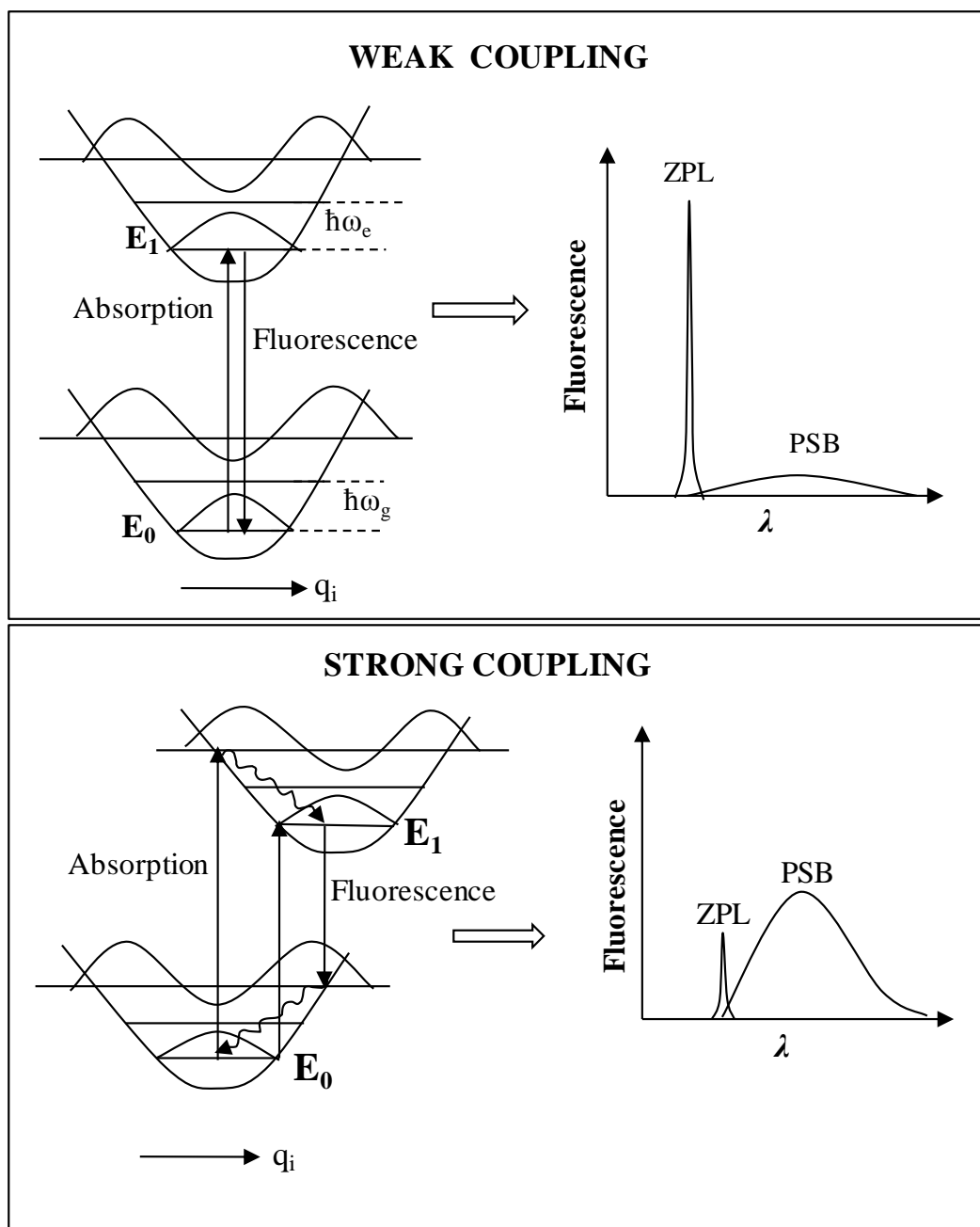
Figure 1-8 Schematic of potential energy curves for weak (upper panel) and strong (lower panel) linear (i.e., \omega_g=\omega_e ) el-ph couplings. Electronic transitions between ground ( E_0 ) and excited ( E_1 ) states are indicated by vertical arrows in accordance with Franck Condon approximation.
