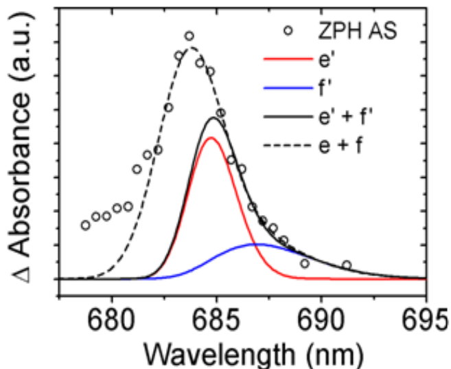
Figure 2-13 Fit of the high-dose ZPH action spectrum (open circles) of CP43' with sub-ensemble SDFs of the two lowest-energy states (A' and B') without inter-monomer EET (curves f and e ) and with inter-monomer EET (curve f' and e' ).
