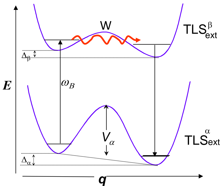
Figure 1-9 Schematic representation of persistent NPHB mechanism. Extrinsic TLS belonging to ground state is labeled as \alpha and \beta , respectively. Asymmetry parameters in ground and excited states are \Delta_{\alpha} and \Delta_{\beta} , respectively, and \omega_B represents burn frequency.
