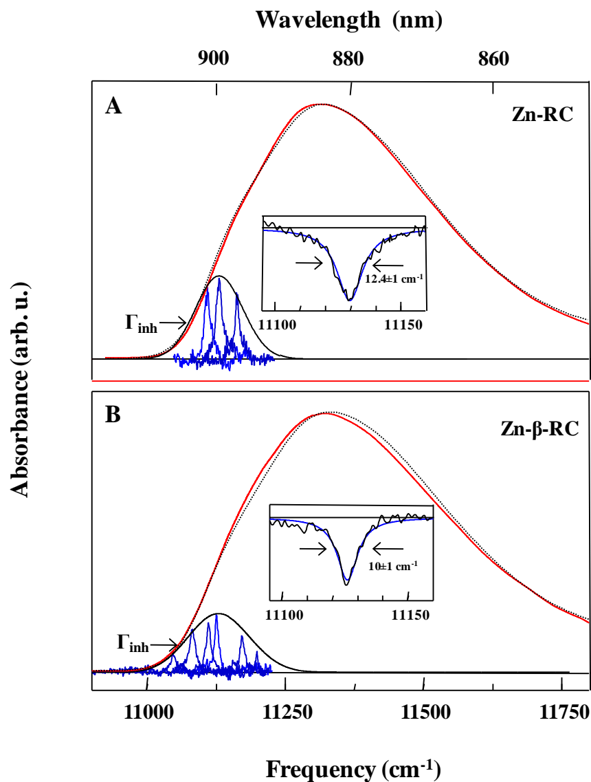
Figure 3-6 Frames A and B show experimental P870 absorption band (black dotted curves) of Zn-RC and Zn-β-RC, respectively. Calculated absorption spectra are shown in red. The blue color sharp spikes in both frames (in the ~11000-11250 cm -1 region) show the inverted ZPHs. The ZPHs were measured under identical conditions ( I = 250 \text{ mW/cm}^2 , read resolution = 1 cm -1 ). The insets show a blowup of the experimental (black) ZPHs obtained with the burn wavelength ( \lambda_B ) of 898.4 nm ( \omega_B = 11131 \text{ cm}^{-1} ) (frame A) and 898.7 nm ( \omega_B = 11127 \text{ cm}^{-1} ) for Zn-RC (frame A) and Zn-β-RC (frame B), respectively. The Lorentzian fits of the ZPHs are shown in blue.
