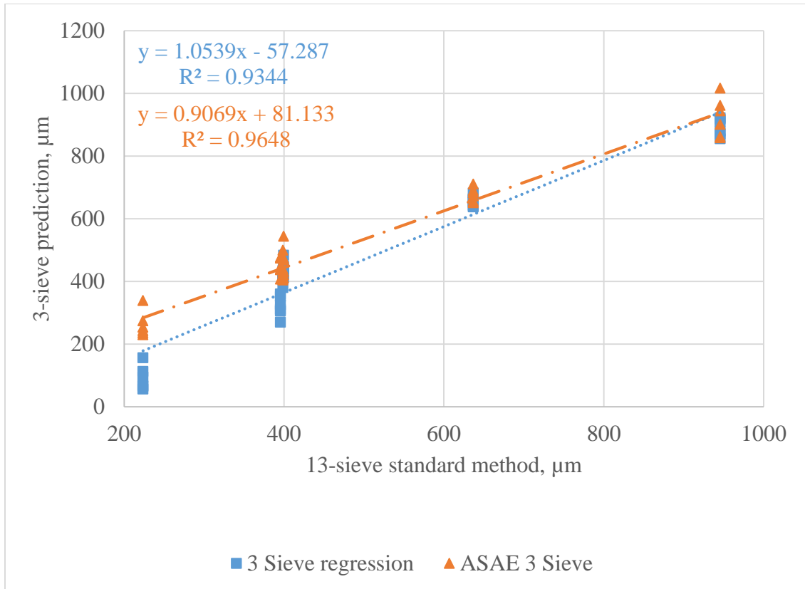
Figure 3.1 Relationship in prediction of geometric mean diameter ( d_{gw} ) using a 3-sieve method compared to ANSI/ASAE Standard 13-sieve method
