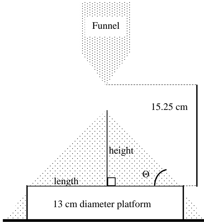
Figure 5.1 Static angle of repose method (adapted from Juliano and Barbosa-Cánovas, 2005) 1
