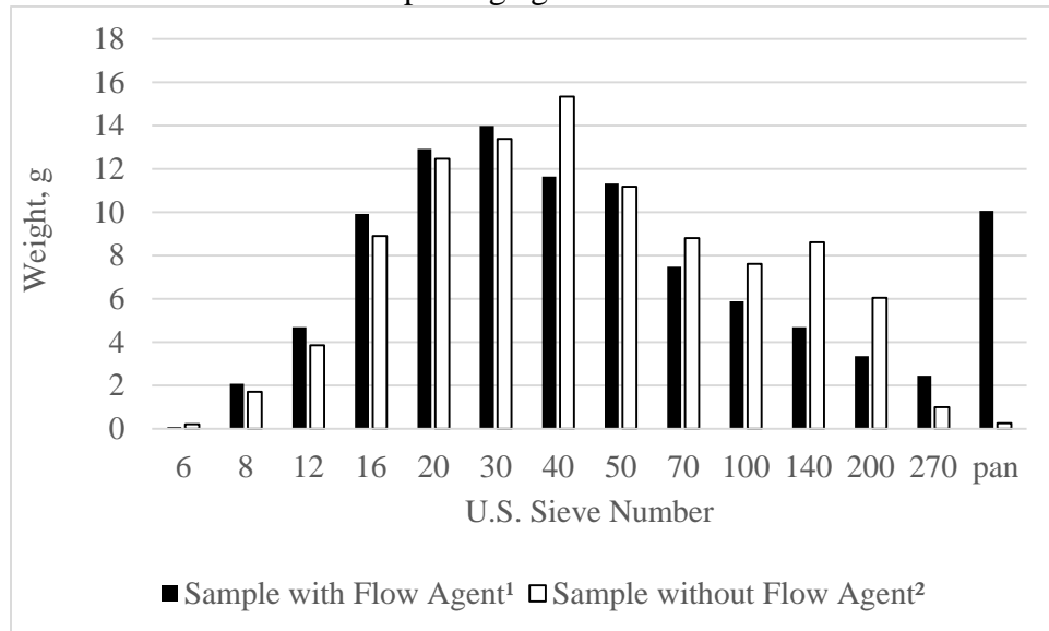
Figure 2.1 Particle size distribution graph of a hammermill ground corn sample with and without the addition of a dispersing agent.
