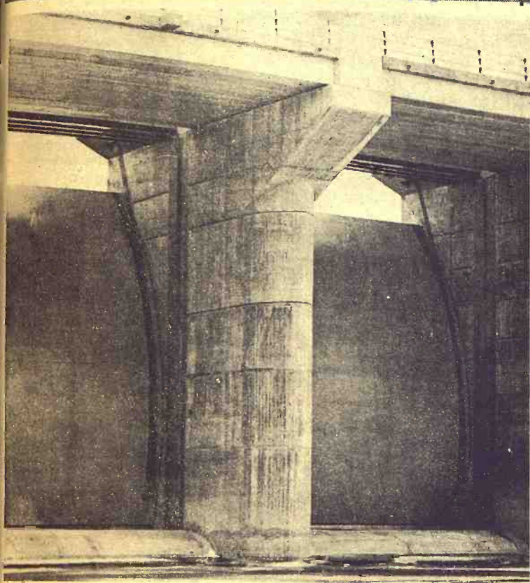
Floodgates are 40 foot by 40 foot.
